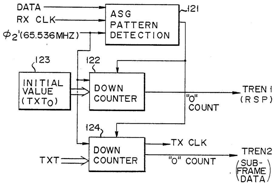
TRANSMISSION TIMING MODULE 96
