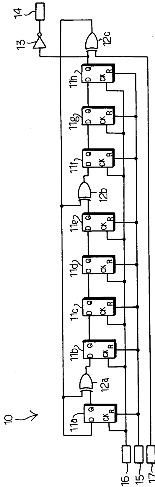
Fig. 2 PRIOR ART
