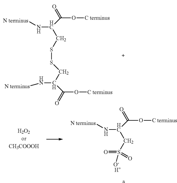
Scheme 1. General representations of (a) oxidation and (b) reduction of disulfide crosslinks in keratin. These reactions cleave the sulfur-sulfur bond in cystine residues, thereby destroying the superstructure and rendering the keratins soluble in the reaction media. The resultant fractions are keratose (a) and keratene (b).
