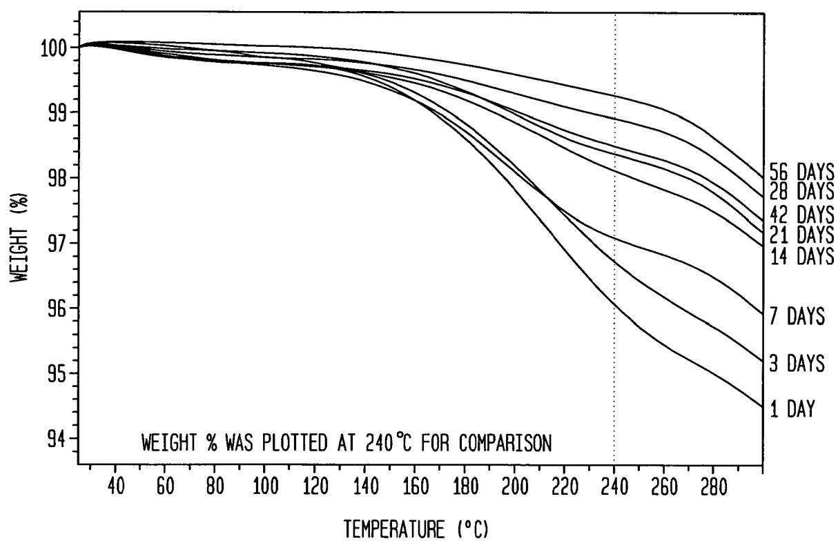
FIG. 9 RESIDUAL COALESCENTS IN DRIED PAINT FILM
