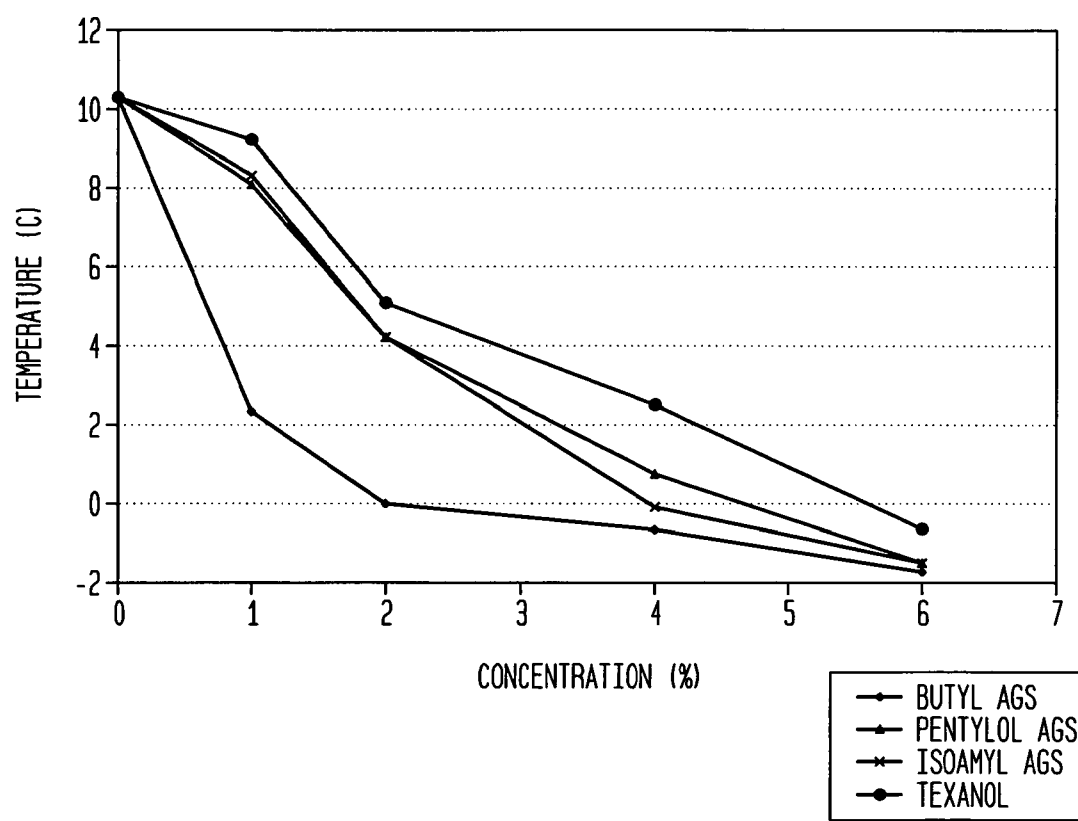
FIG. 5 EFFECT OF AGS BLENDS ON MFFT IN A VINYL/ACRYLIC LATEX
