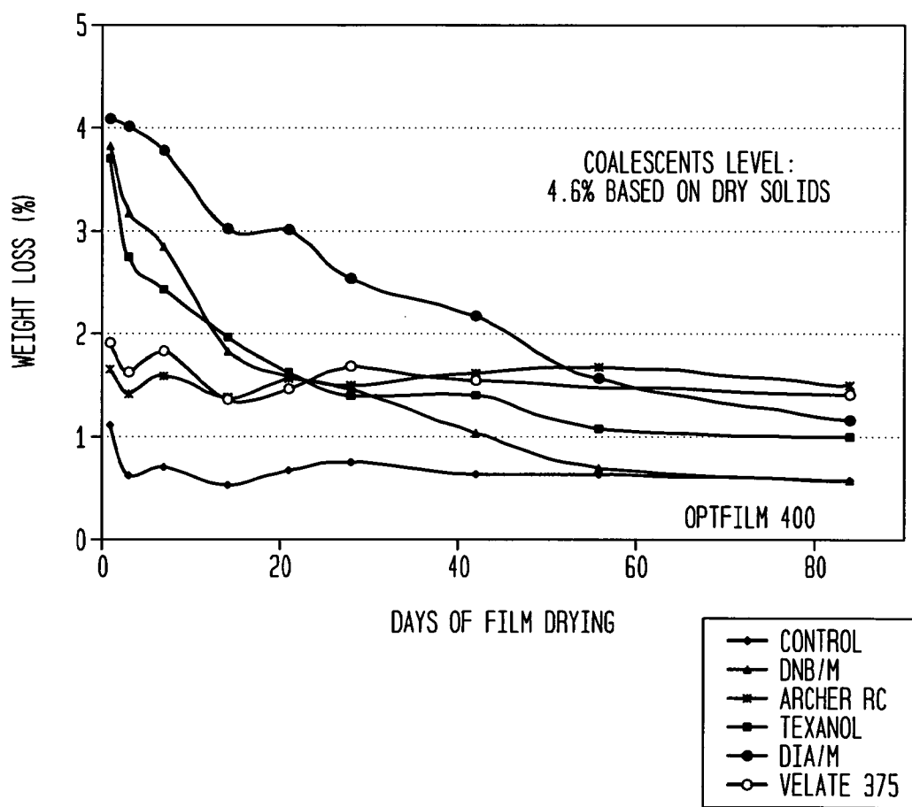
FIG. 10 RESIDUAL COALESCENT IN PAINT FILM - TGA ANALYSIS
