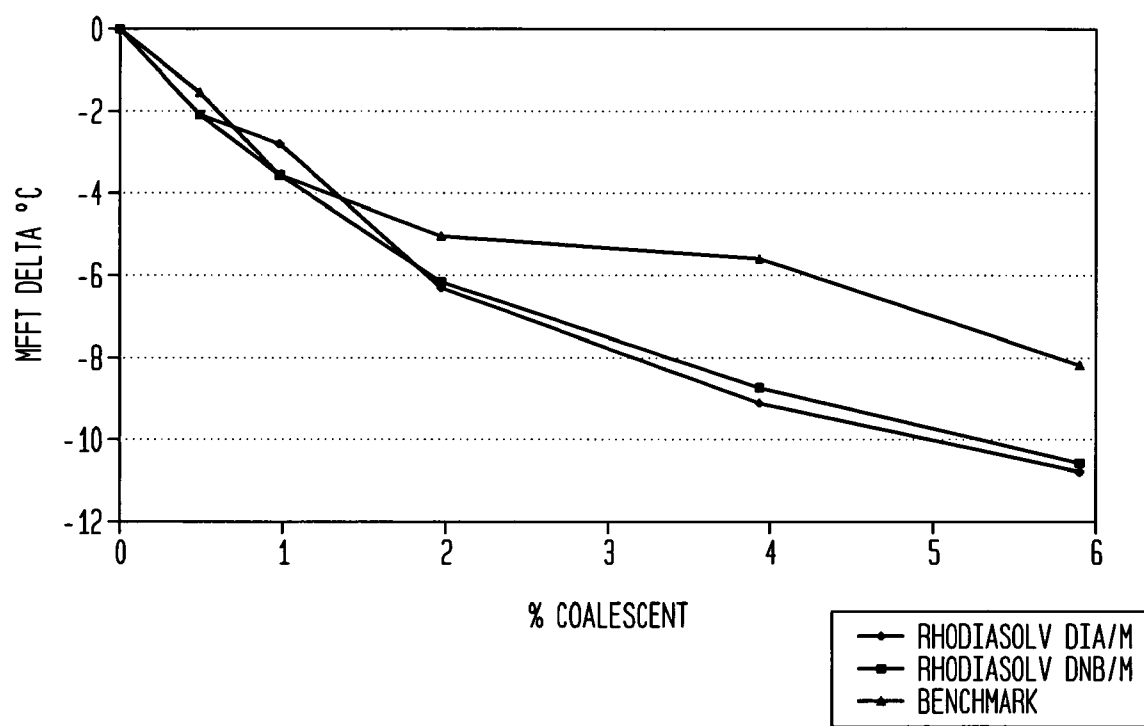
FIG. 7 MFFT RESULTS FOR VINYL-ACRYLIC RESIN
