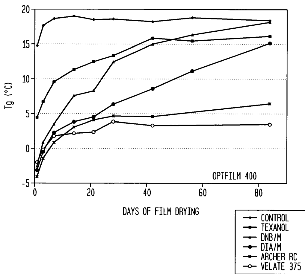
FIG. 11 RESIDUAL COALESCENT IN PAINT FILM - DSC ANALYSIS
