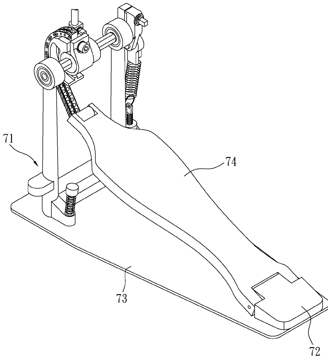
FIG. 10 PRIOR ART
