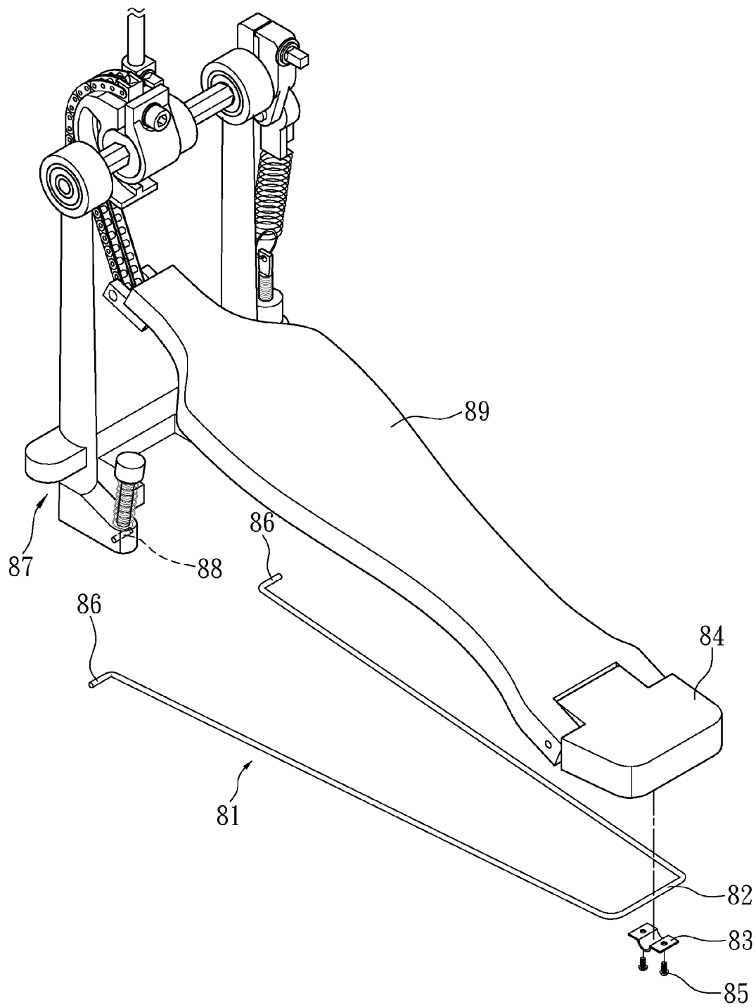
FIG. 11 PRIOR ART
