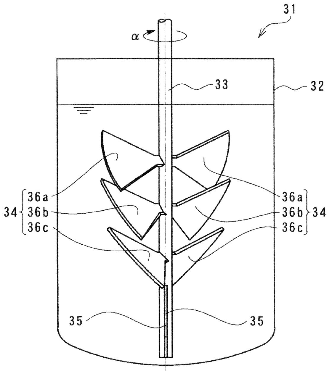
Fig.33(Prior Art)
