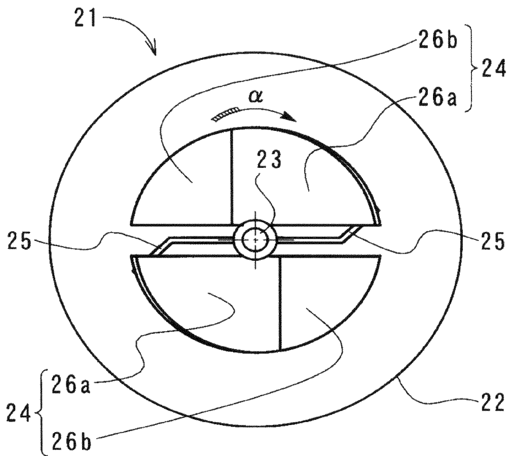
Fig.31(Prior Art)
