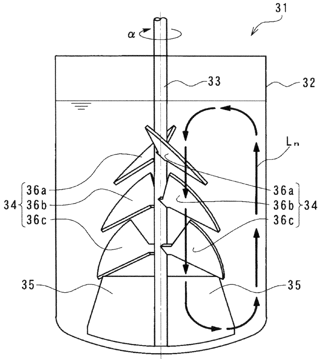
Fig.32(Prior Art)
