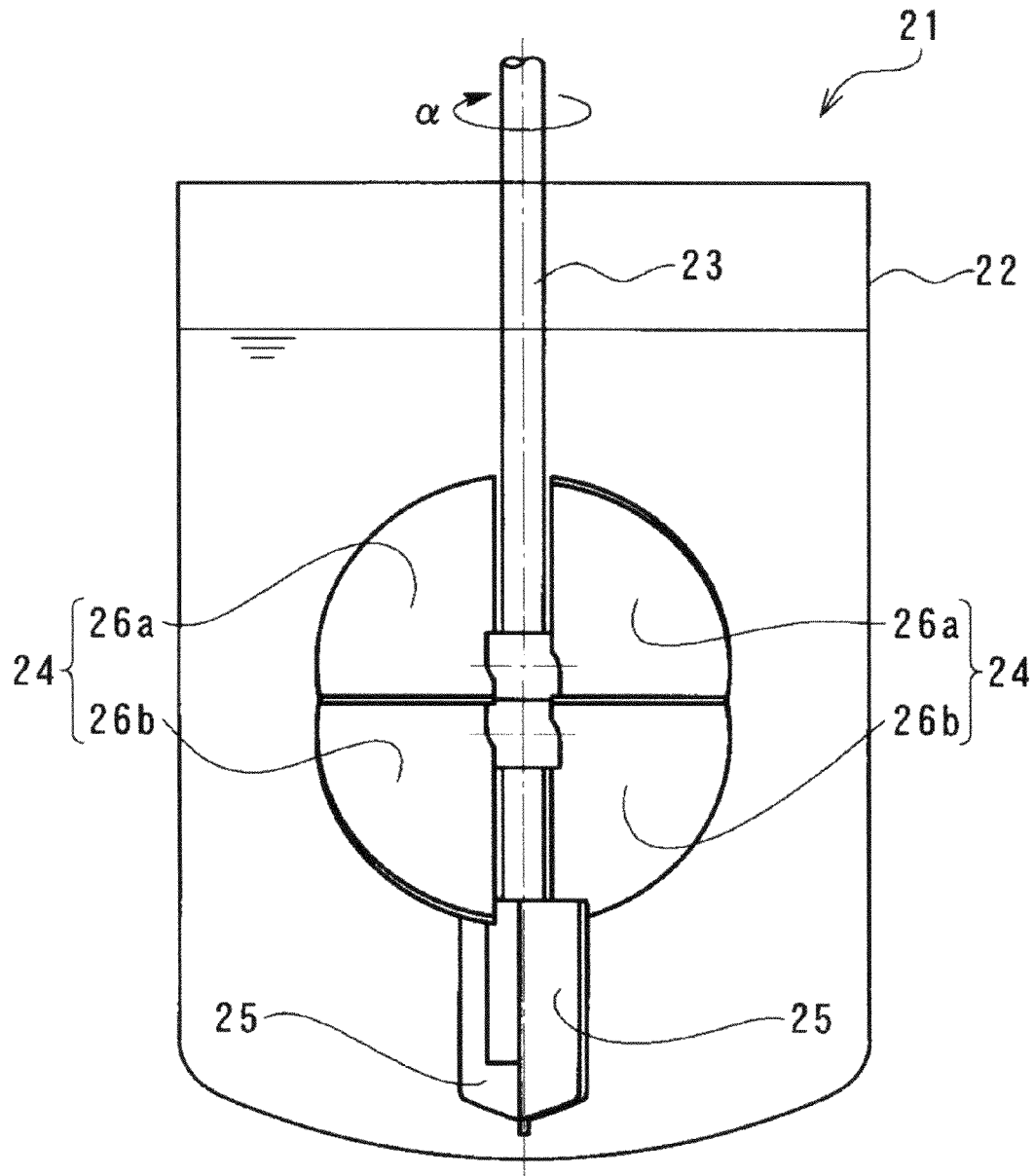
Fig.30(Prior Art)
