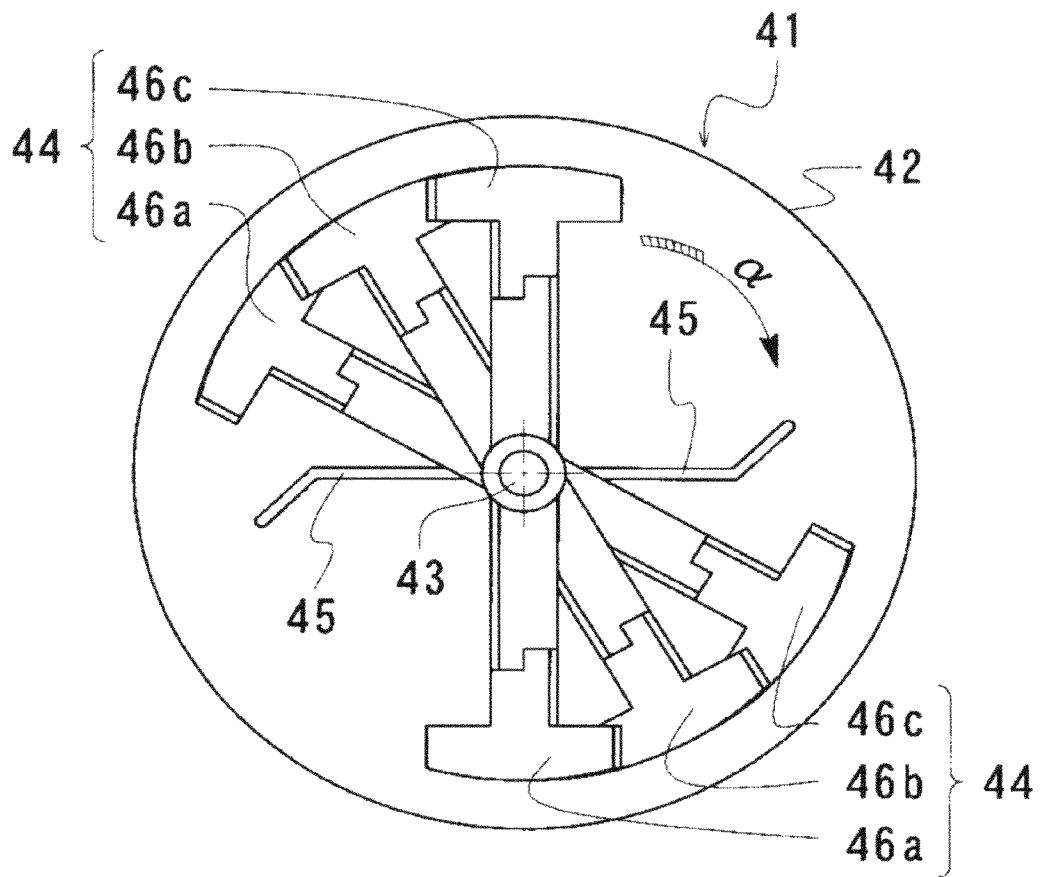
Fig.37(Prior Art)
