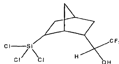
2,2,2-Trifluoro-1-(6-trichlorosilanyl- bicyclo[2.2.1]hept-2-yl)-ethanol
