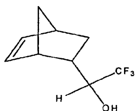
1-Bicyclo[2.2.1]hept-5-en-2-yl -2,2,2-trifluoro-ethanol
