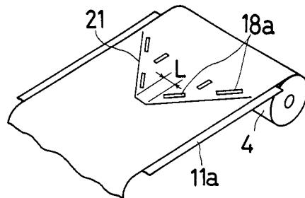
PRIOR ART FIG. 10
