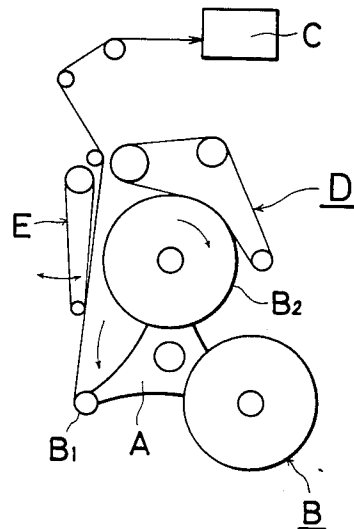
PRIOR ART FIG. 11
