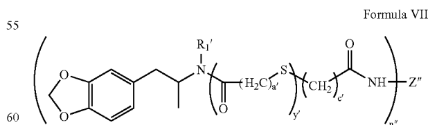
Formula VII
