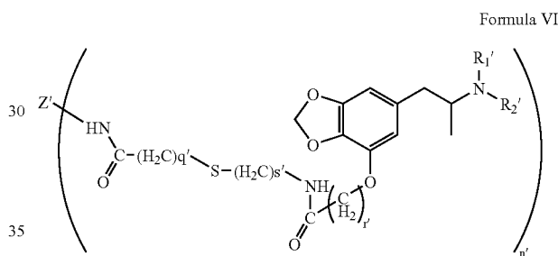
Formula VI
