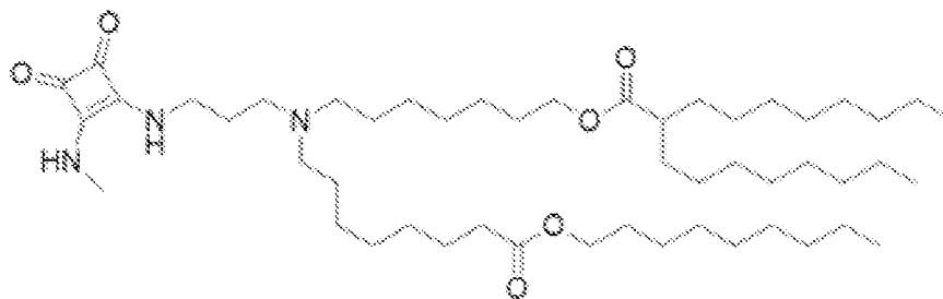
(A6),
