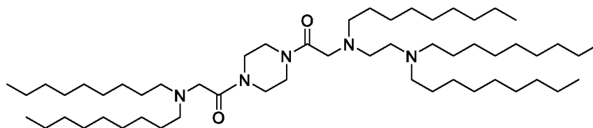
Compound (A),
