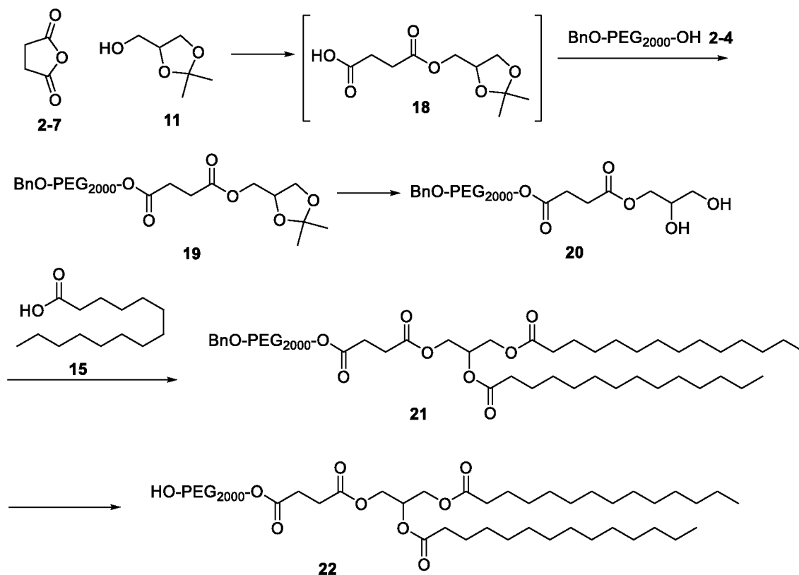
Scheme 7
