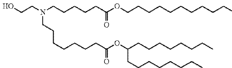
Compound (C),
