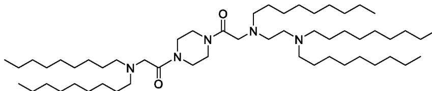
Compound (A),
