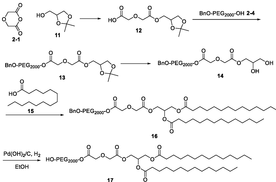
Scheme 6
