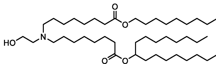
Compound (B),
