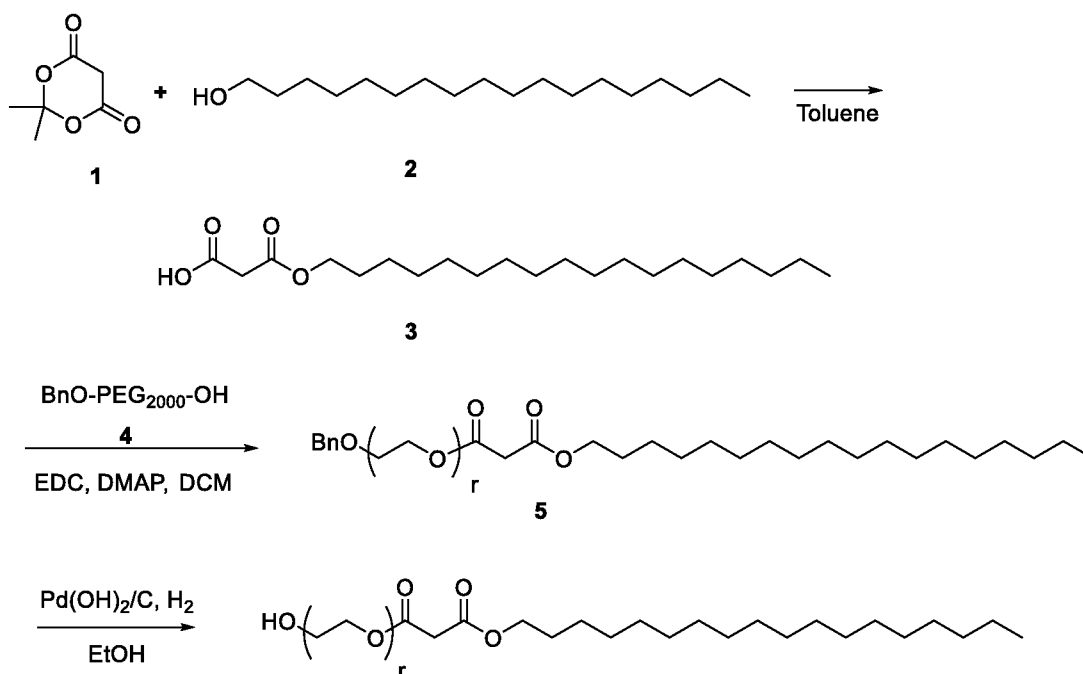
Scheme 10
