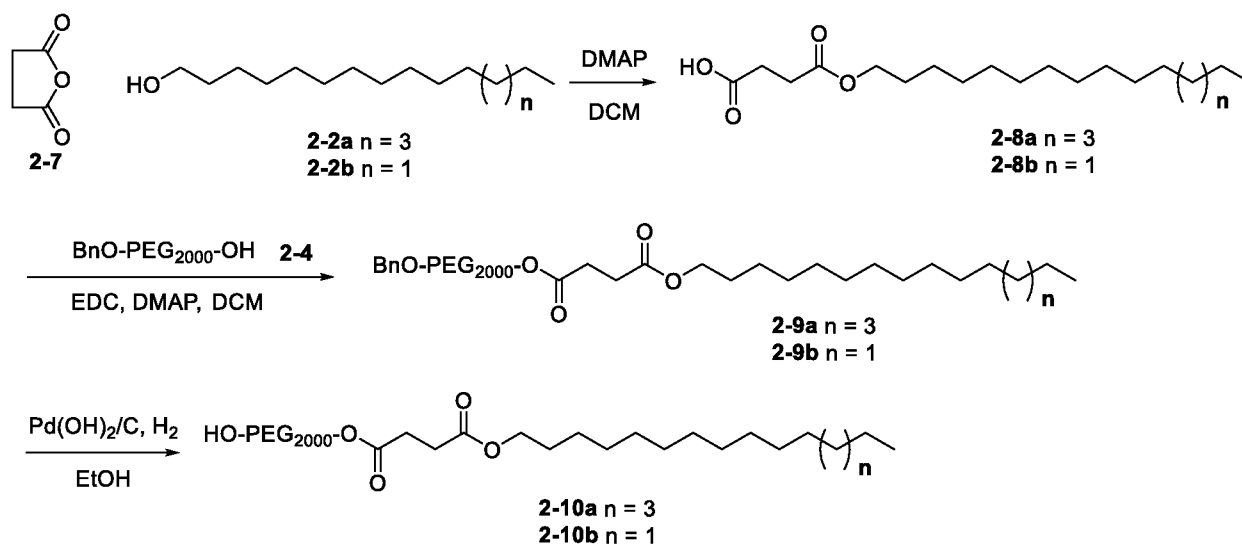
Scheme 5
