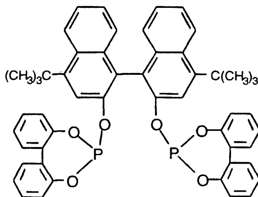
Ligand C
