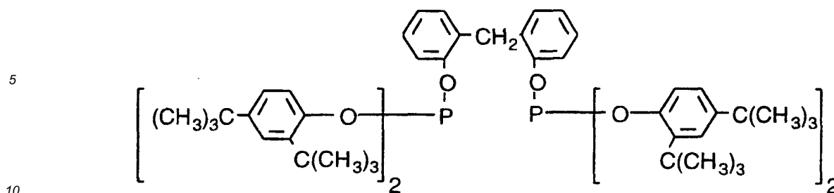
Ligand U
