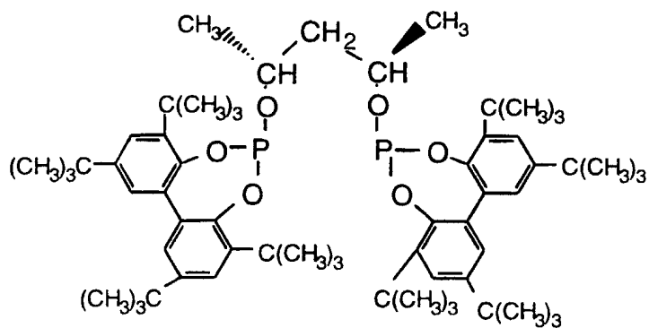
Ligand H
