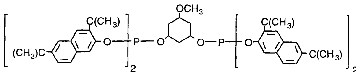
Ligand S
