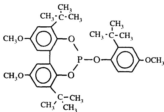
Ligand A
