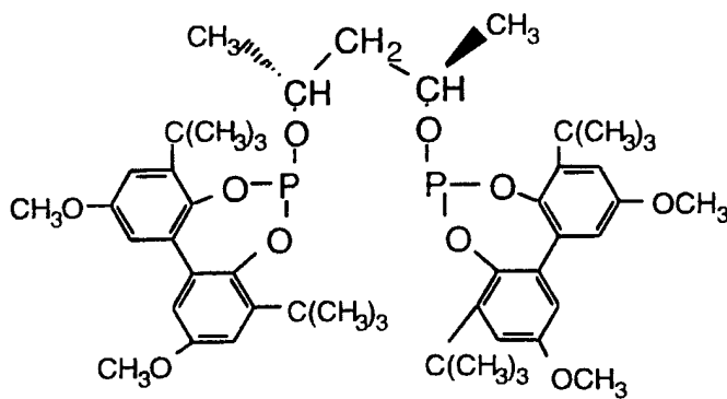
Ligand M
