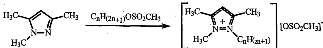
Scheme 6. An alternate synthesis of pyrazolium ionic liquids.
