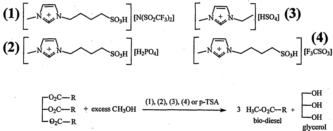
Reaction 3, catalysts used in the acid catalysed transesterification of lard.
