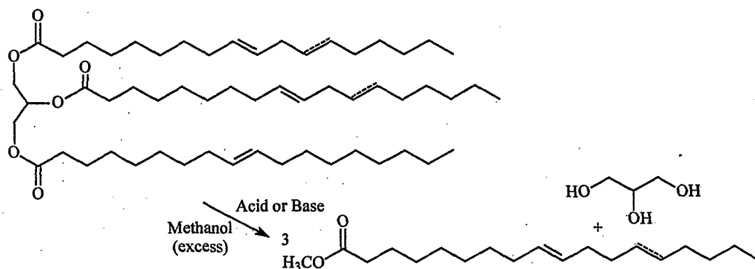
Scheme 2, The acid and base catalysed transesterification of triglycerides, the major constituent of animal fat.
