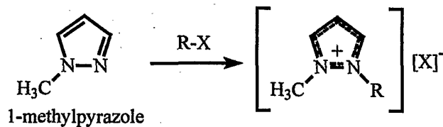
Scheme 4. Synthesis of 1-methylpyrazolium ionic liquids.
