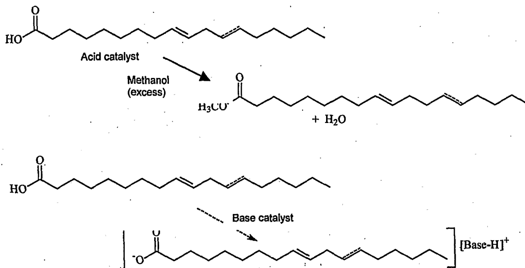
Scheme 1, The acid and base catalysed esterification of fatty acids.
