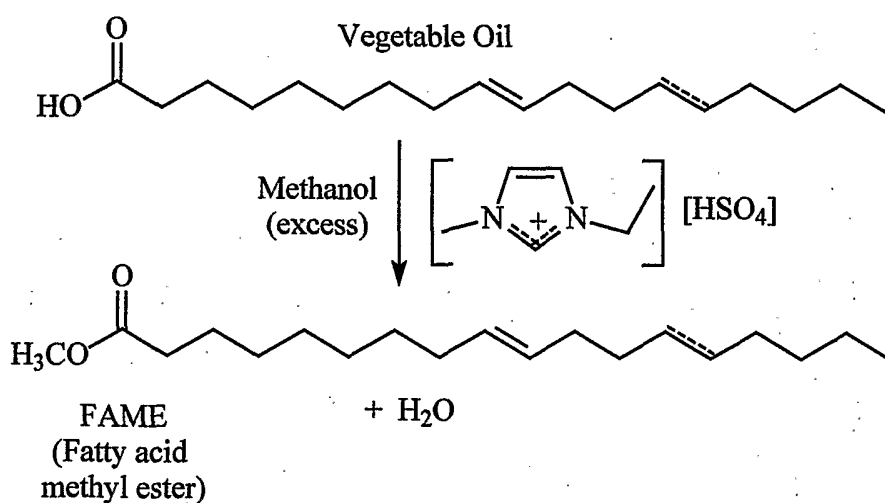
Reaction 1a, The esterification of vegetable oil (Prialene 6927) with [emim][HSO 4 ].
