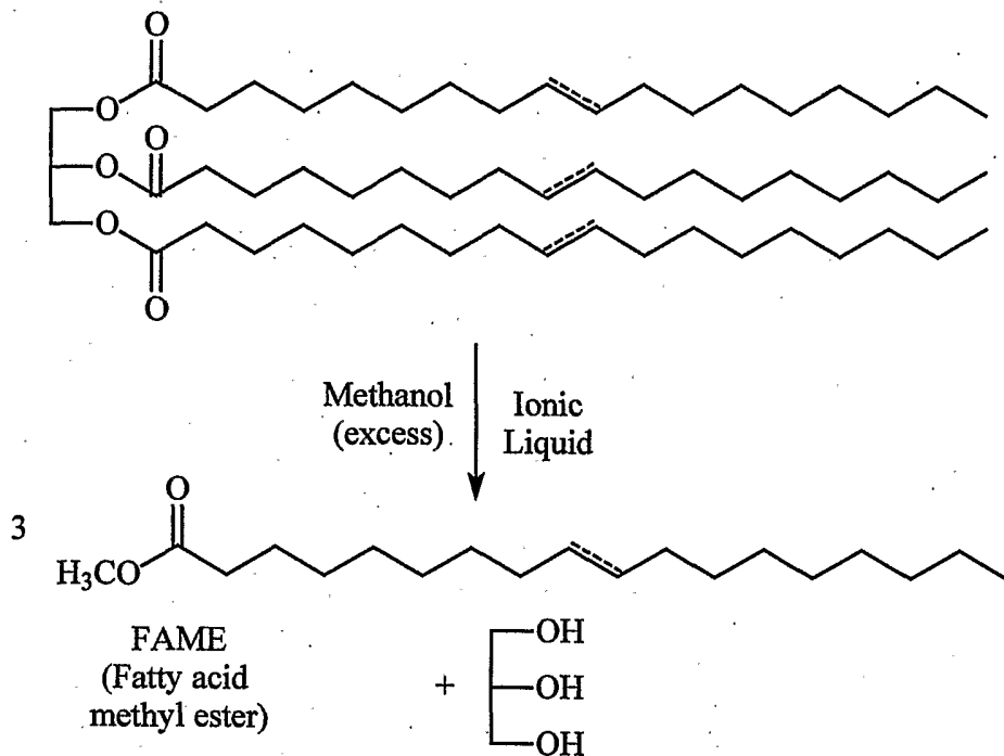
Reaction 2, The animal fat transesterification reaction in ionic liquids
