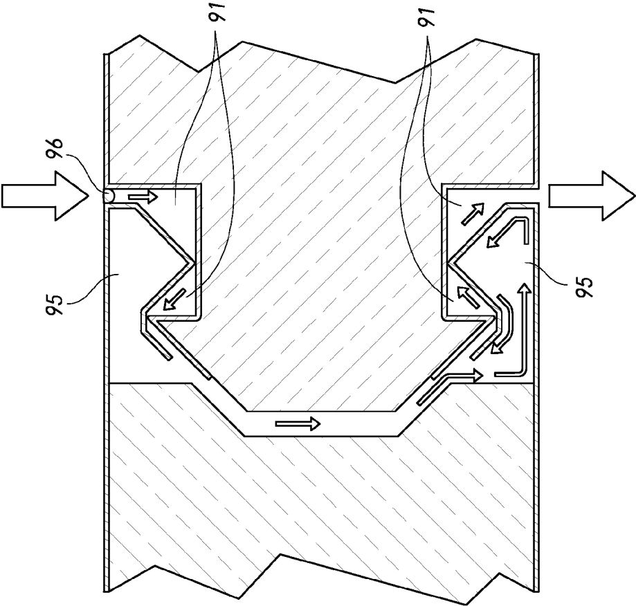
FIG. 10 (PRIOR ART)
