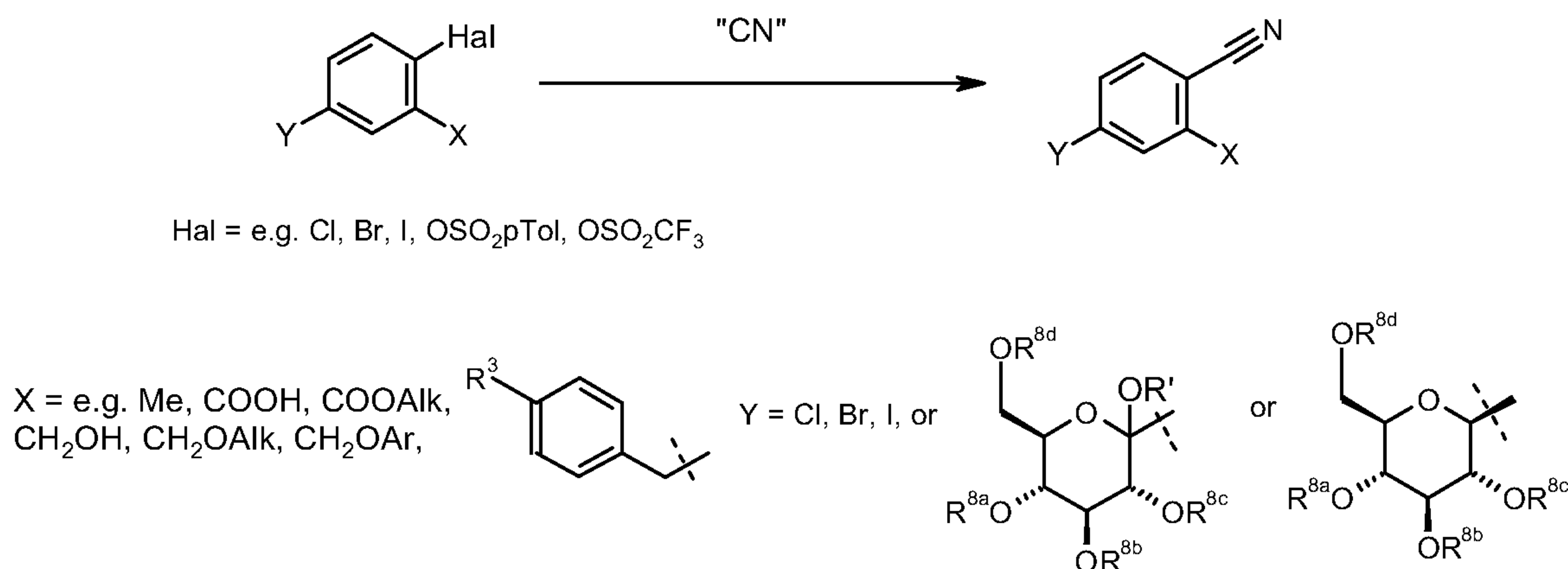
Scheme 5: Introduction of the Cyano Moiety
