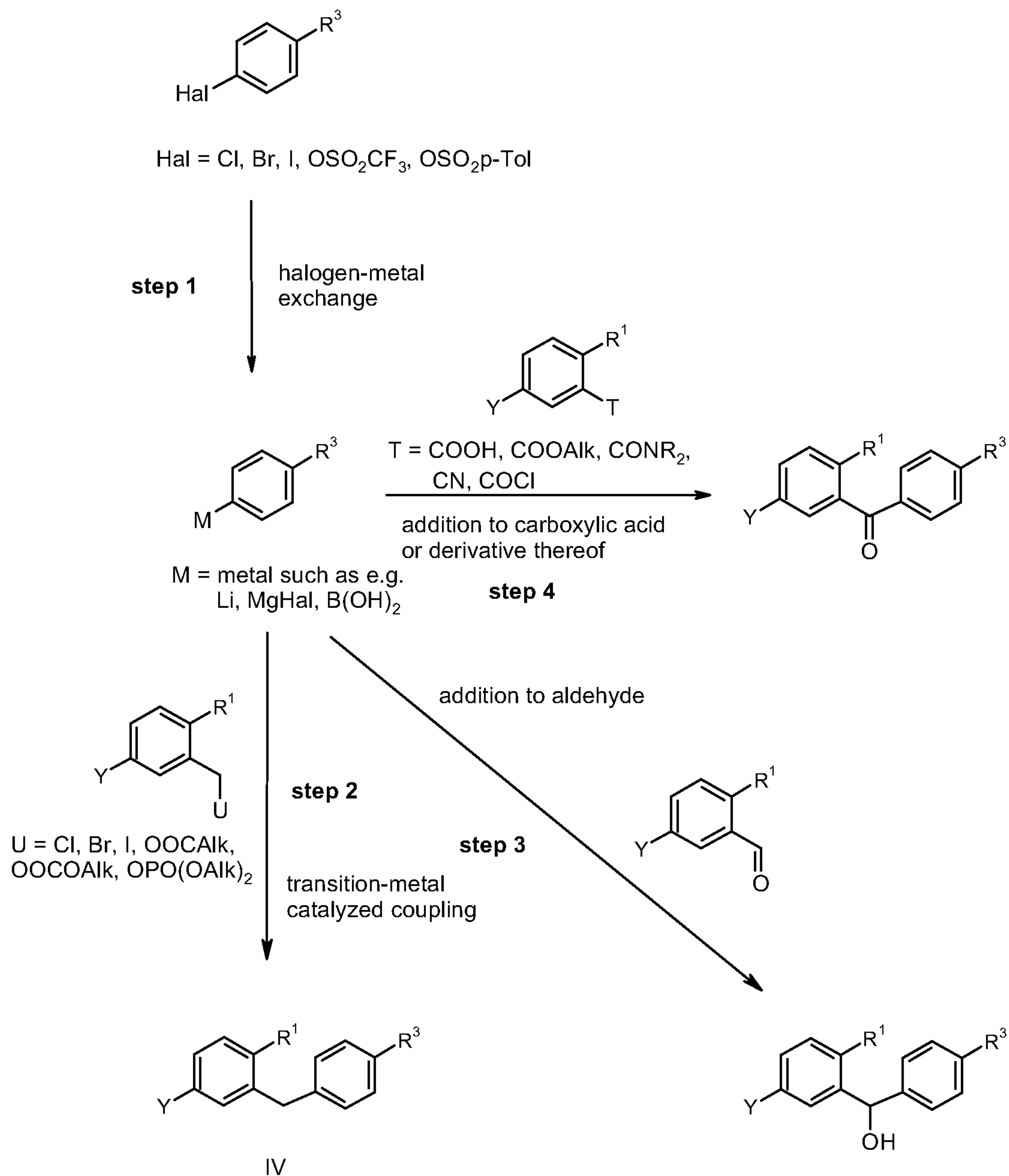
Scheme 4: Synthesis of Diarylmethane Unit and Possible Precursor Compounds thereof
