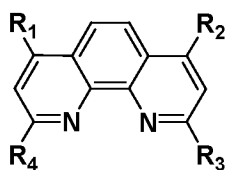
1, 10-phenanthroline derivatives
