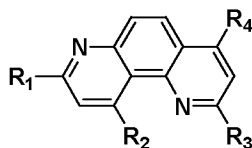
1, 7-phenanthroline derivatives
