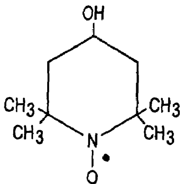
4-Hydroxy-TEMPO
