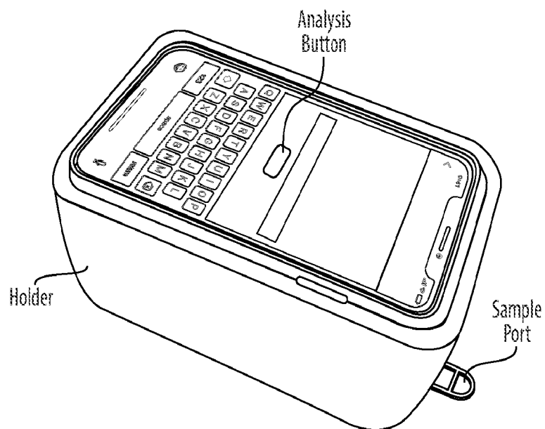
Figure 2 -- Holder
