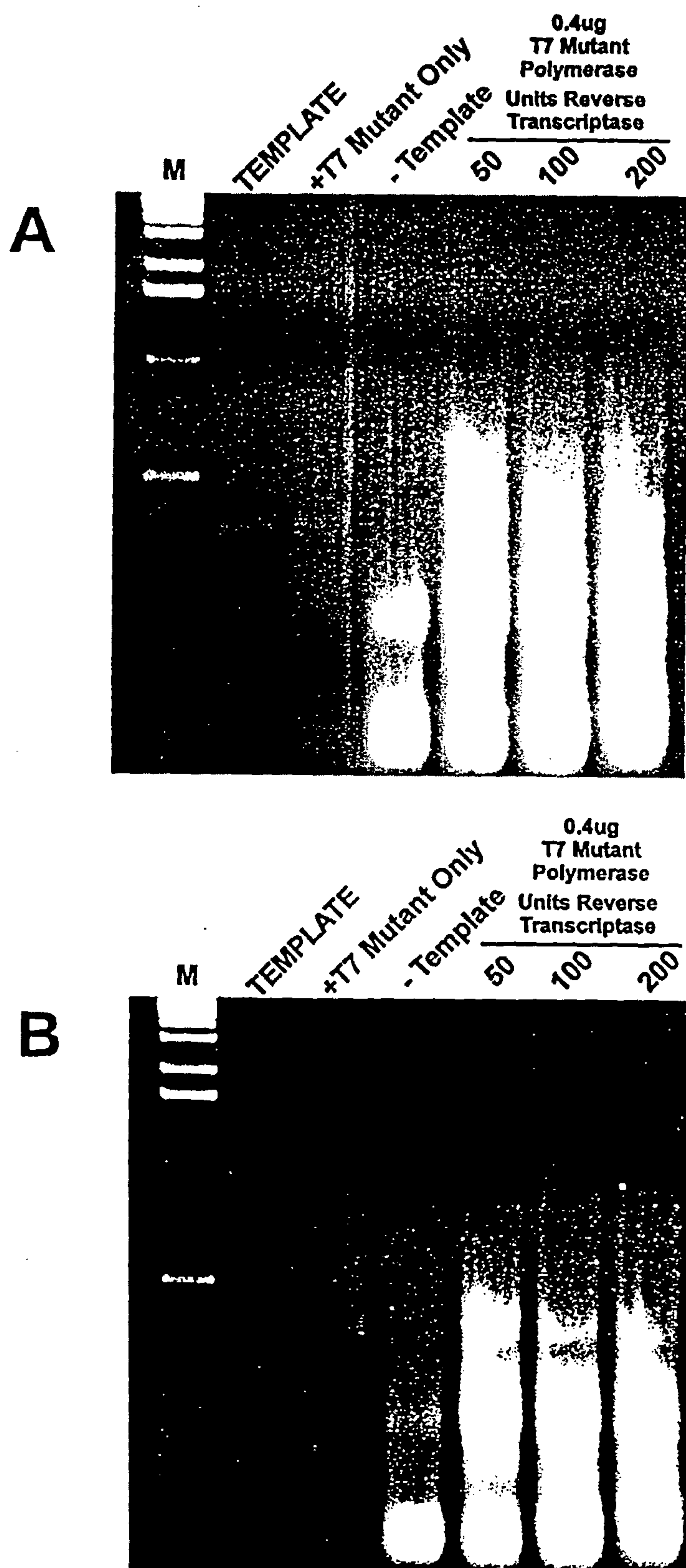
Figure 8 Agarose Gel Electrophoretic Analysis of Amplification Products
