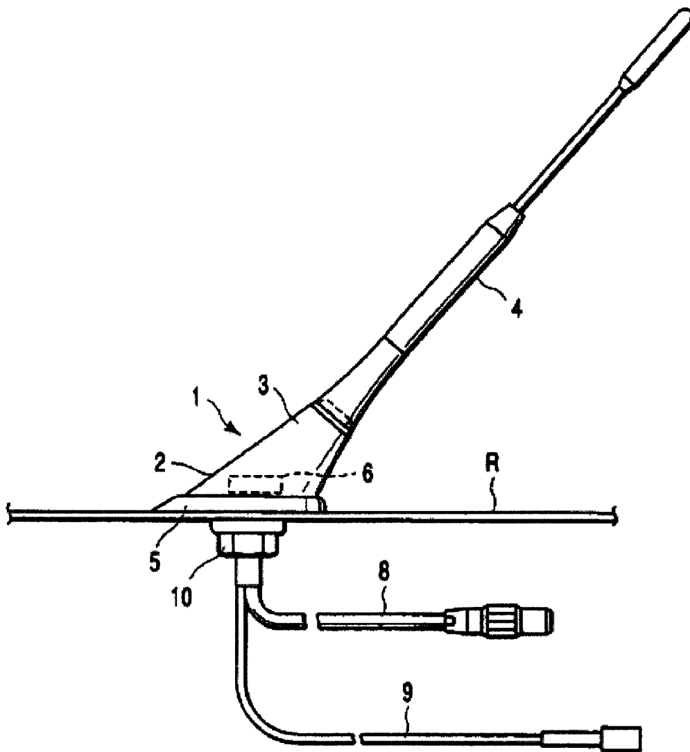
FIG. 14 PRIOR ART
