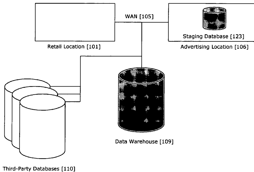
FIG 2. Media Targeting Data Warehouse
