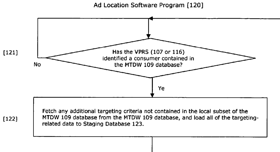
FIG 5. Staging Database Generation Software Flowchart
