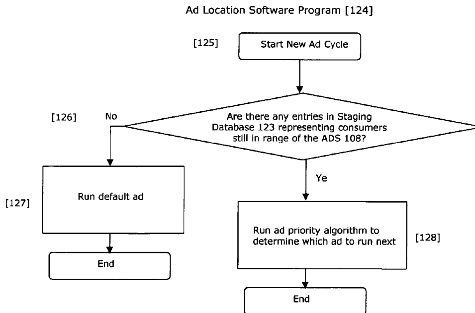
FIG 6. Media Scheduling Engine Software Flowchart
