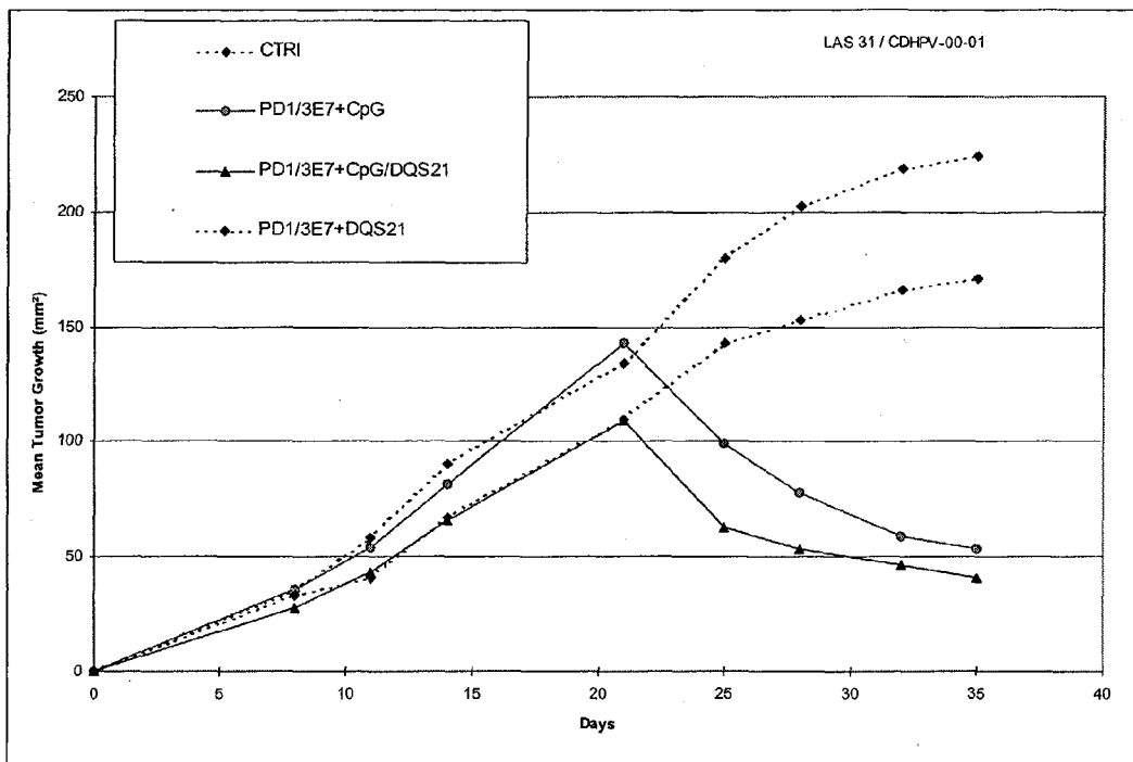
Figure 12: Tumour-growth per group of 10 animals over time
