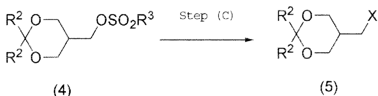
Reaction Scheme-6
