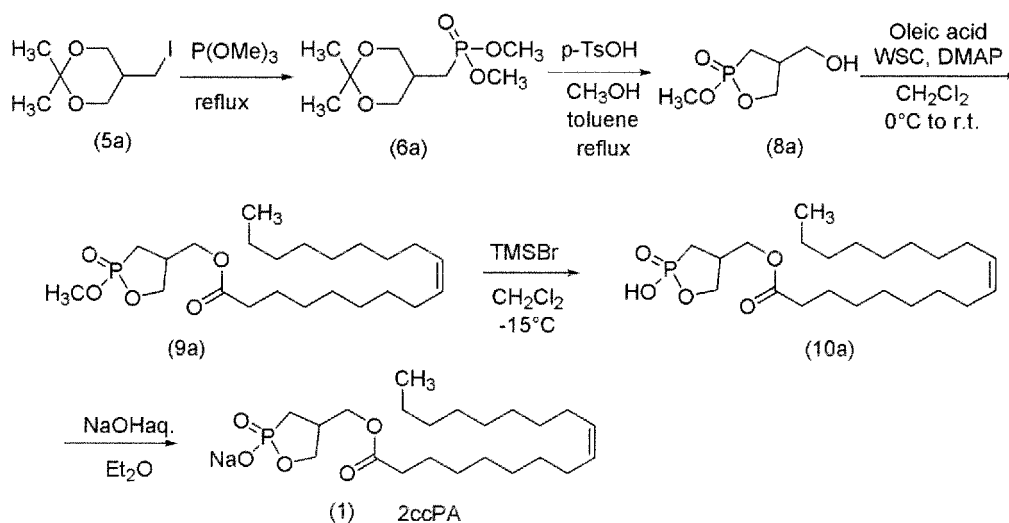
Reaction Scheme-1
