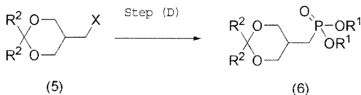
Reaction Scheme-8
