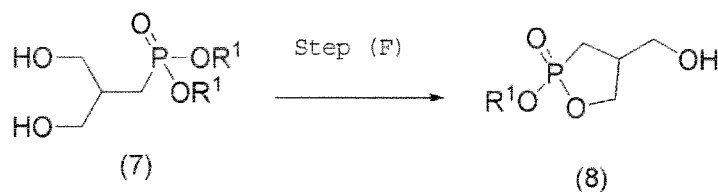
Reaction Scheme-10
