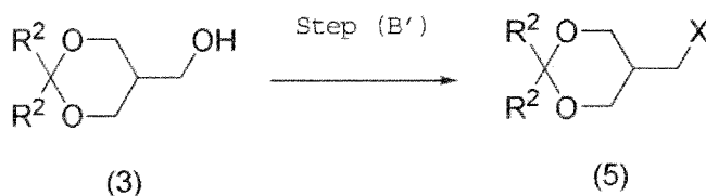
Reaction Scheme-7
