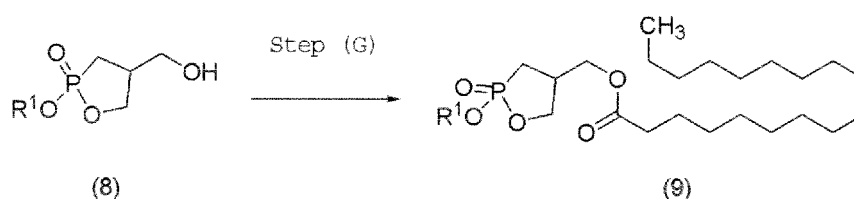
Reaction Scheme-11
