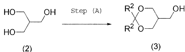
Reaction Scheme-4
