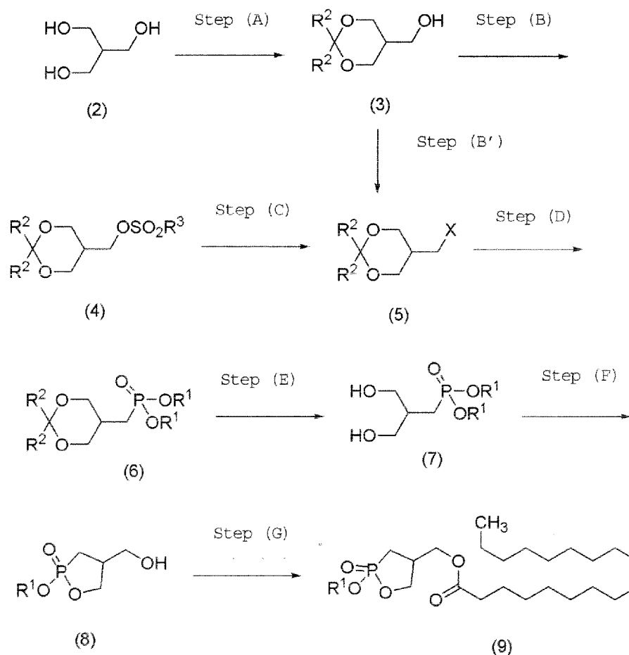
Reaction Scheme-3
