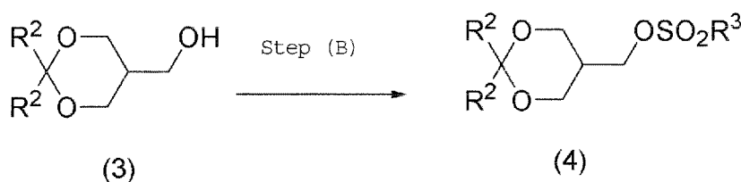
Reaction Scheme-5
