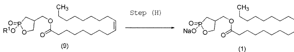
Reaction Scheme-2
