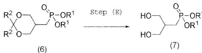
Reaction Scheme-9
