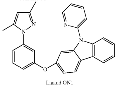
Ligand ON1
