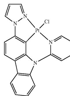
PtN1pyCl
