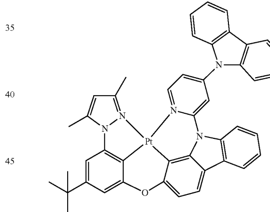
PtON1-Cab-tBu
