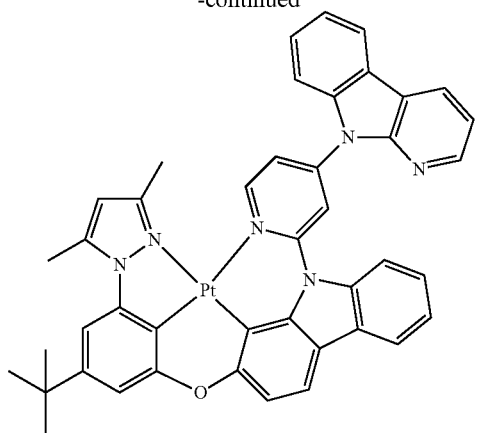
PtON1-N-Cab-tBu
