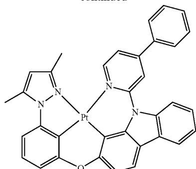
PtON1Ph
