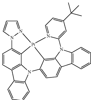
PtN1N-tBu
