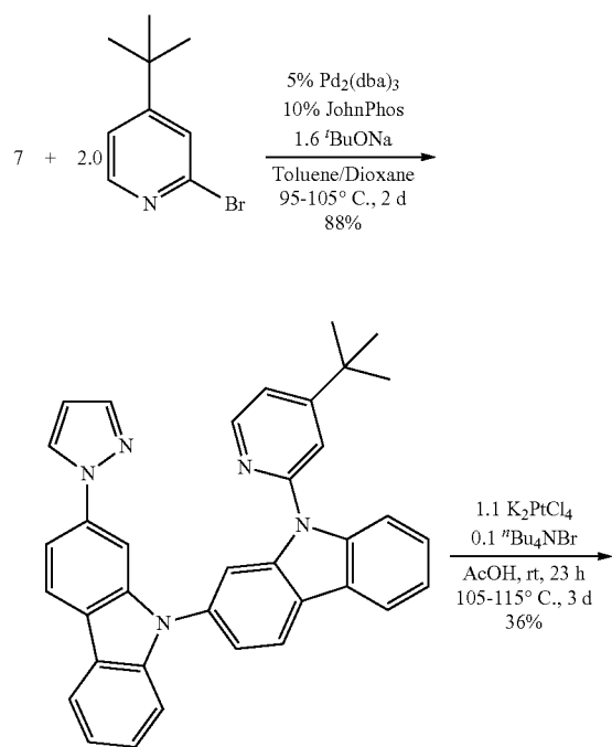
Ligand N1N-tBu
