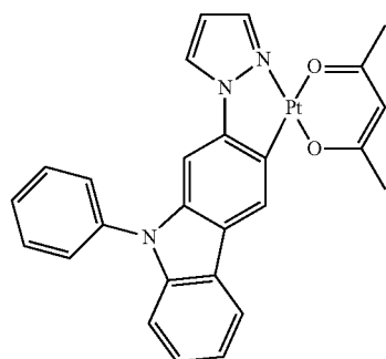
PtN1(acac)
