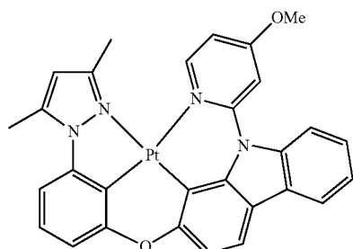
PtON1OMe
