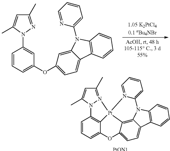
PtON1
