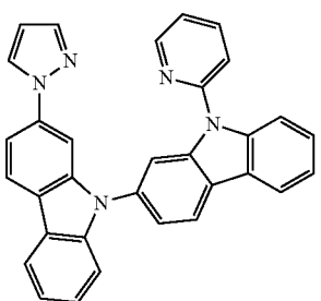
Ligand N1N
