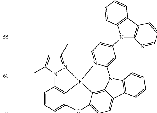
PtON1-N-Cab
