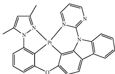
PtON1N
