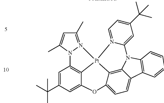
PtON1-di-tBu
