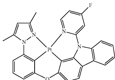
PtON1F
