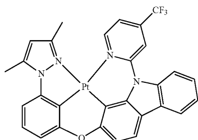
PtON1CF 3
