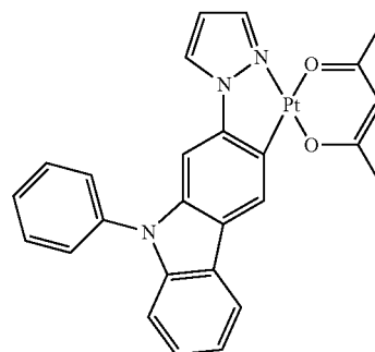
PtN1(acac)
