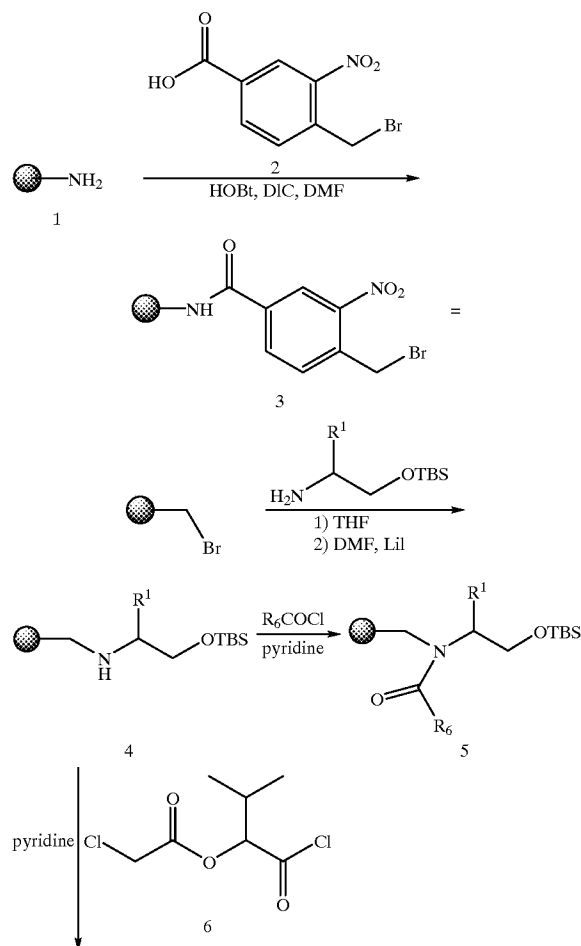
Scheme 1 Hydroxyphosphonate synthesis
