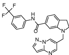
Example 63
