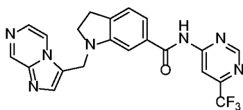
Example 88
