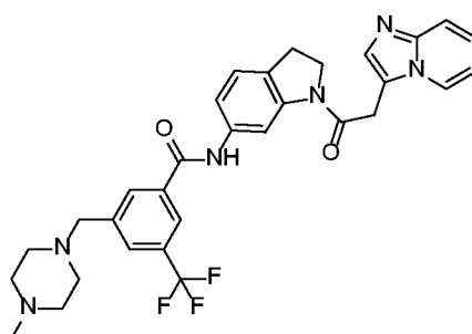
Example C2
