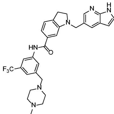
Example 9
