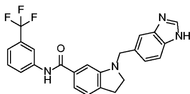
Example 60
