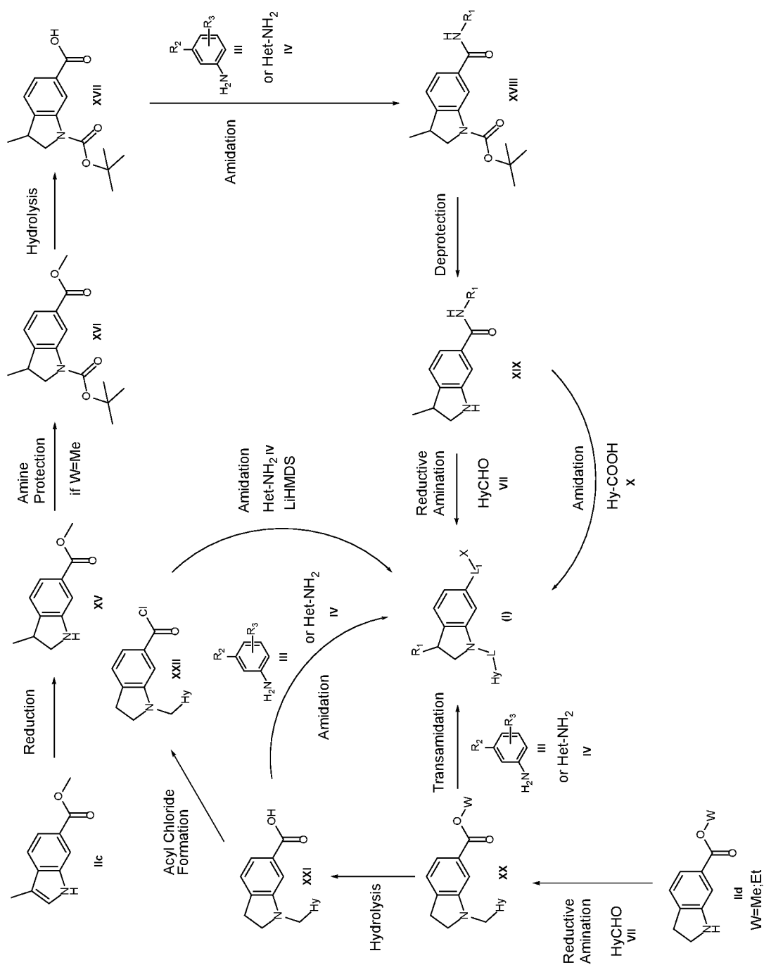
Scheme 2
