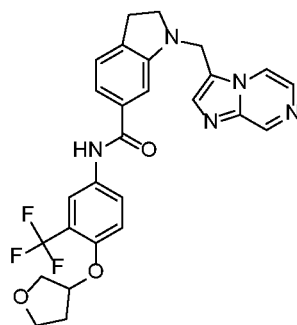
Example 47
