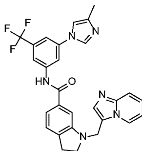
Example 1
