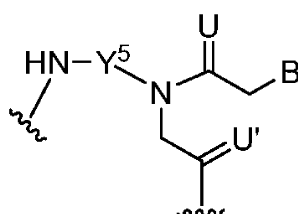
Formula V'.
