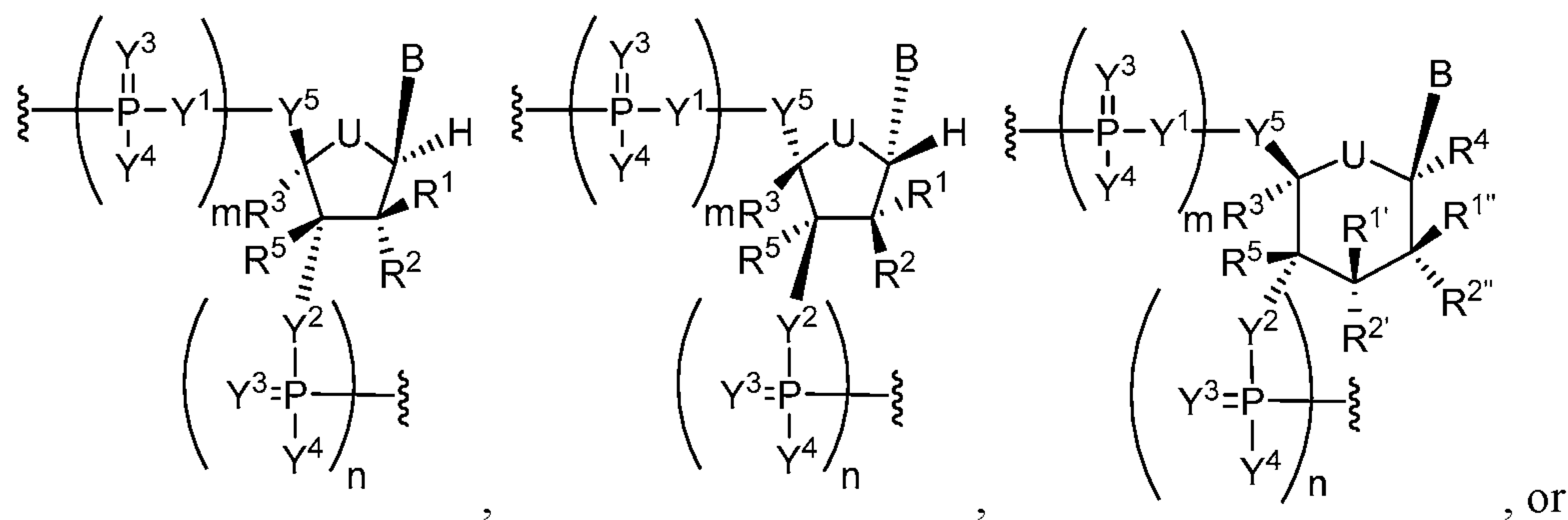
Formula II'
