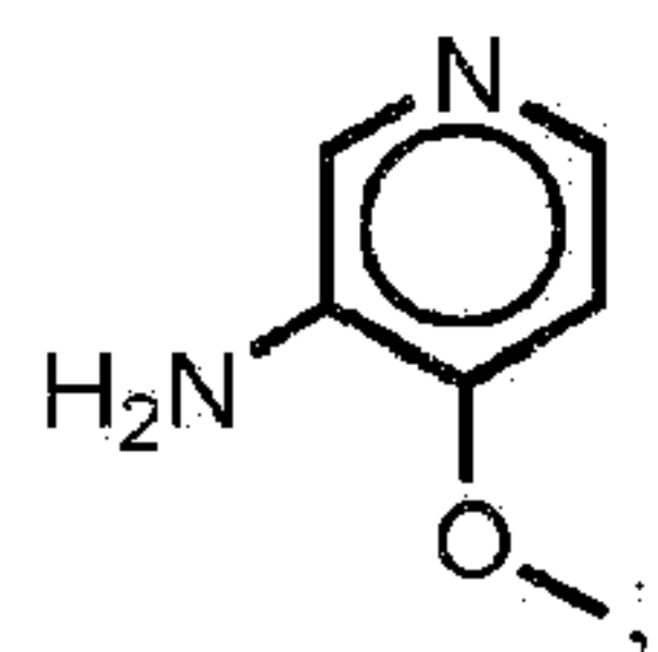
4-methoxypyridin-3-amine:
