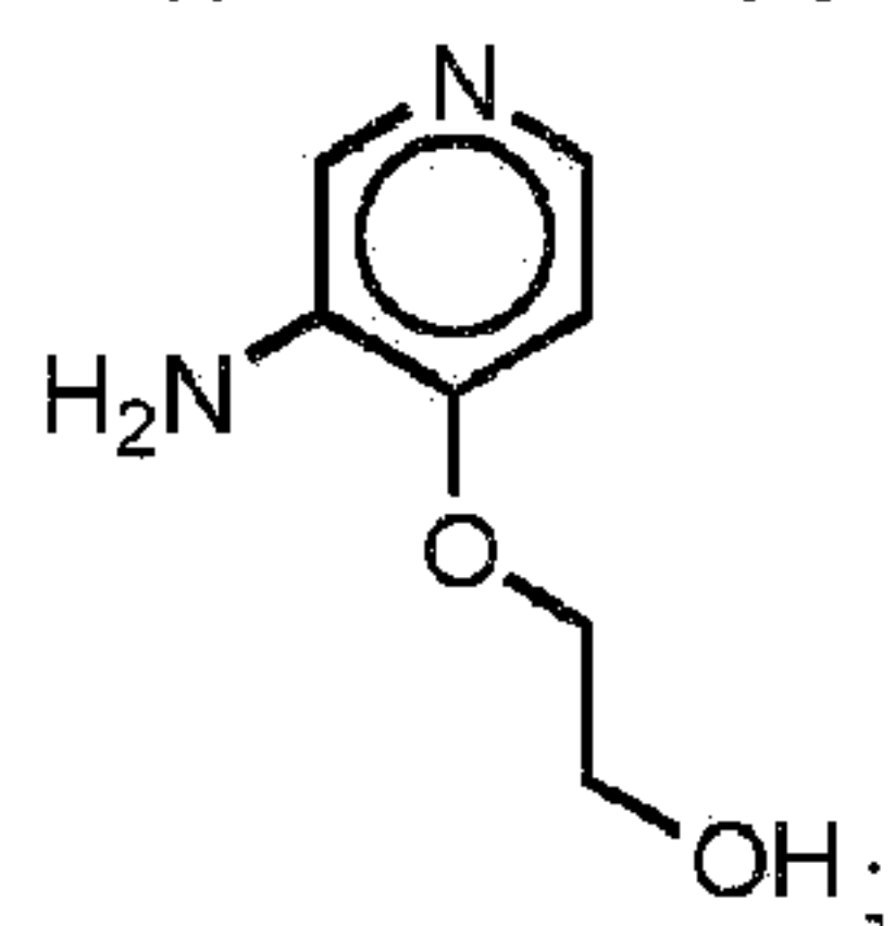
2-((3 -aminopyridin-4-yl)oxy)ethanol:
