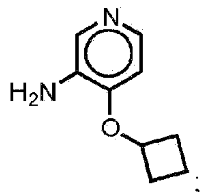
4-cyclobutoxypyridin-3-amine:
