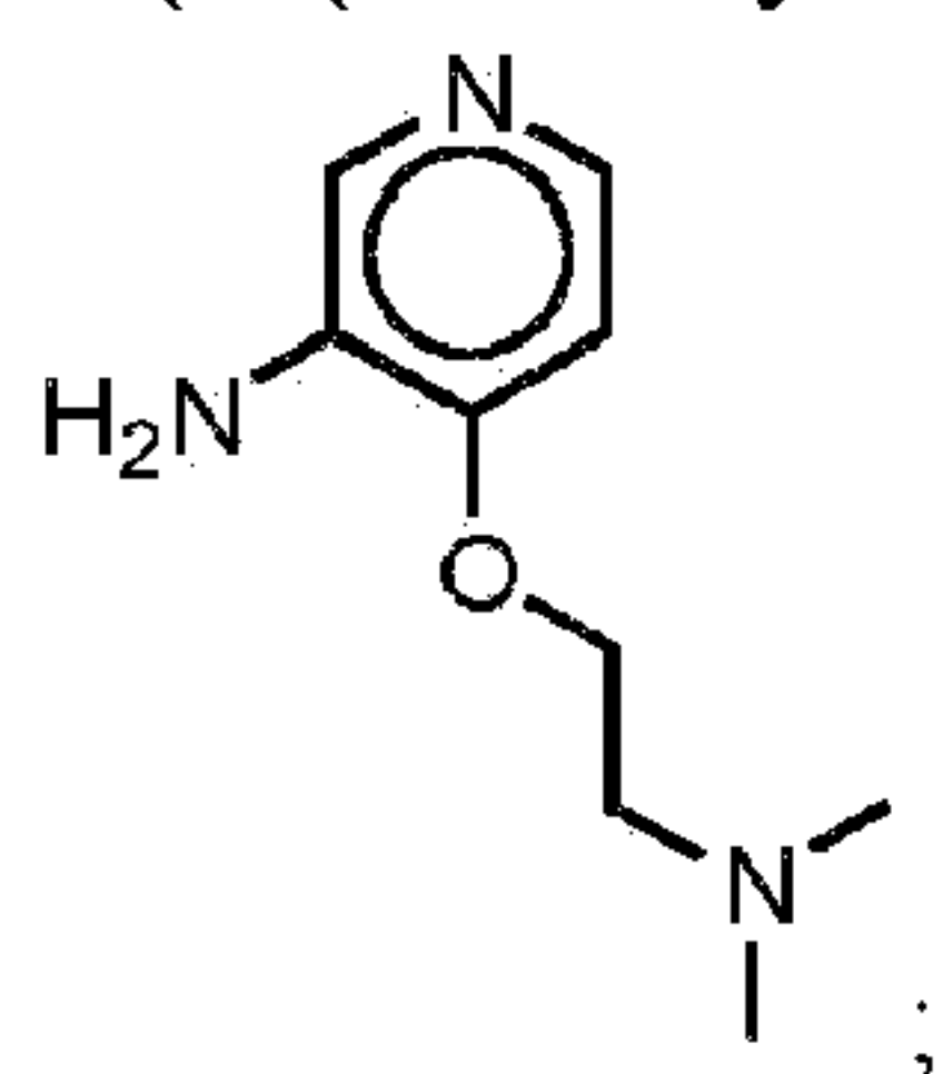
4-(2-(dimethylamino)ethoxy)pyridin-3-amine:
