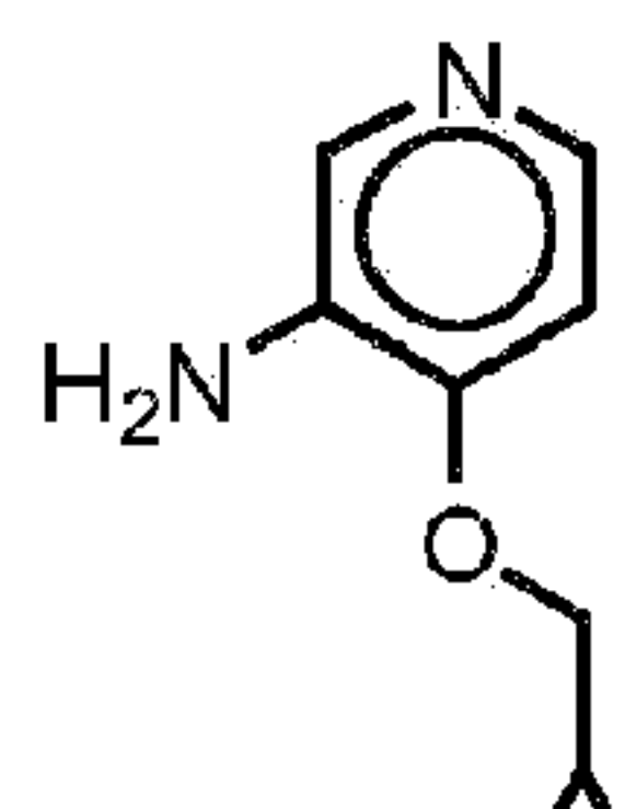
4-(cyclopropylmethoxy)pyridin-3-amine:
