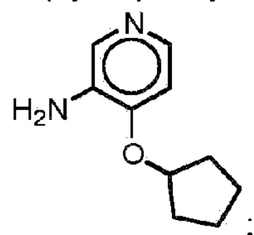
4-(cyclopentyloxy)pyridin-3-amine:
