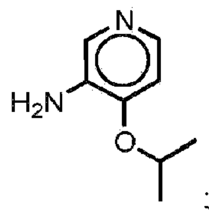
4-isopropoxypyridin-3-amine:
