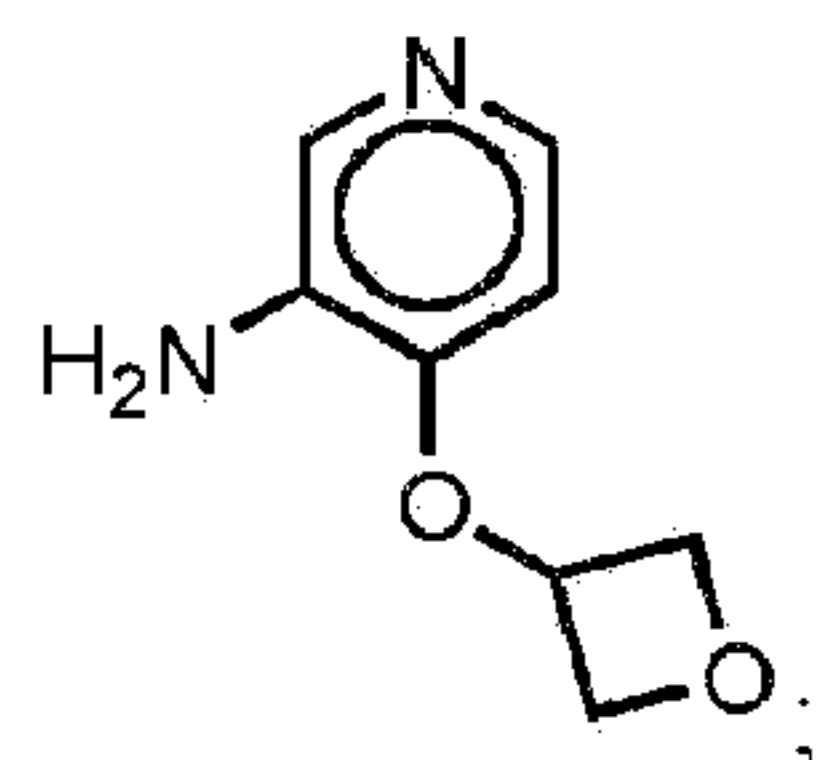
4-(oxetan-3-yl)pyridin-3-amine:
