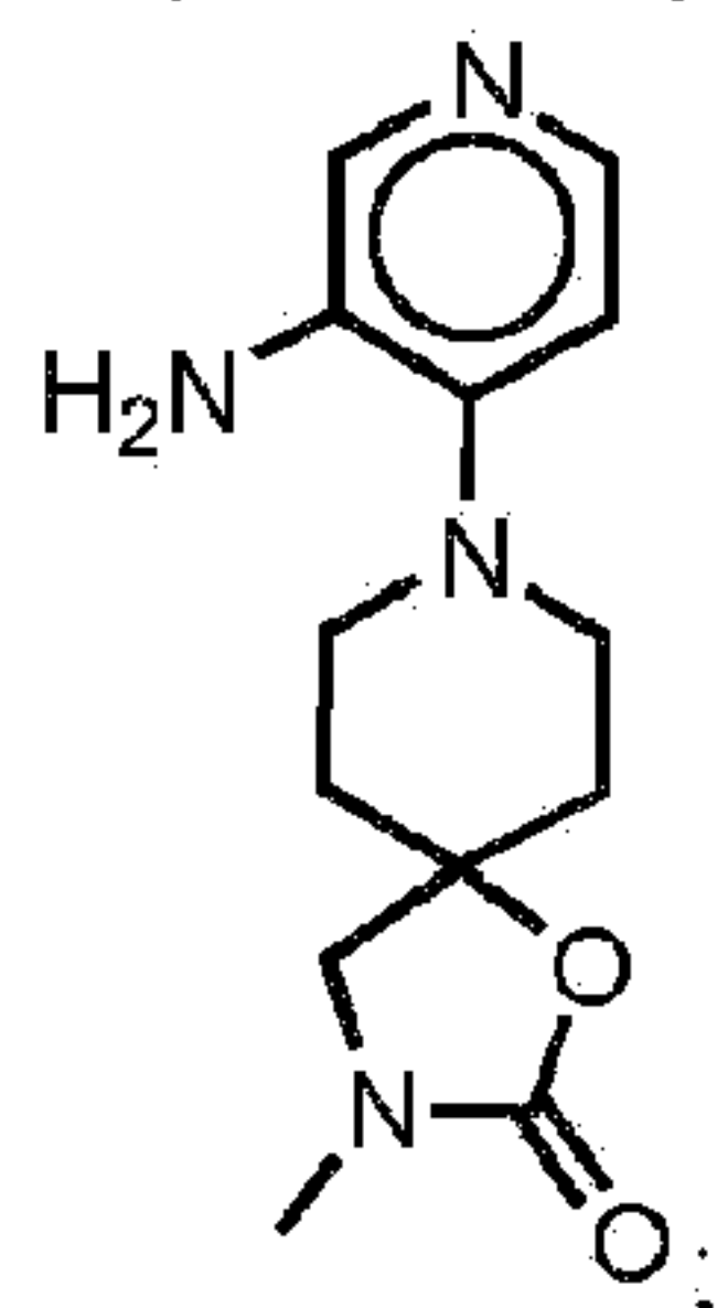
8-(3-aminopyridin-4-yl)-3-methyl-1-oxa-3,8-diazaspiro[4.5]decan-2-one:
