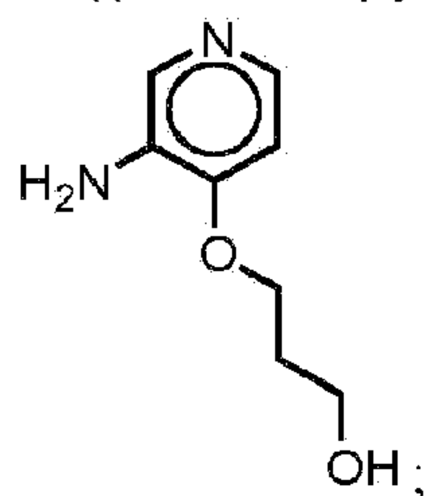
3 -((3 -aminopyridin-4-yl)oxy)propan-1 -ol:
