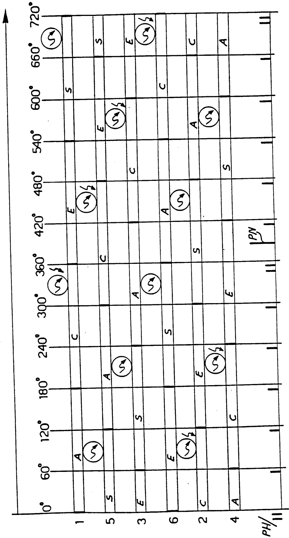
FIG. 5 - 6 CYLINDER ENGINE
