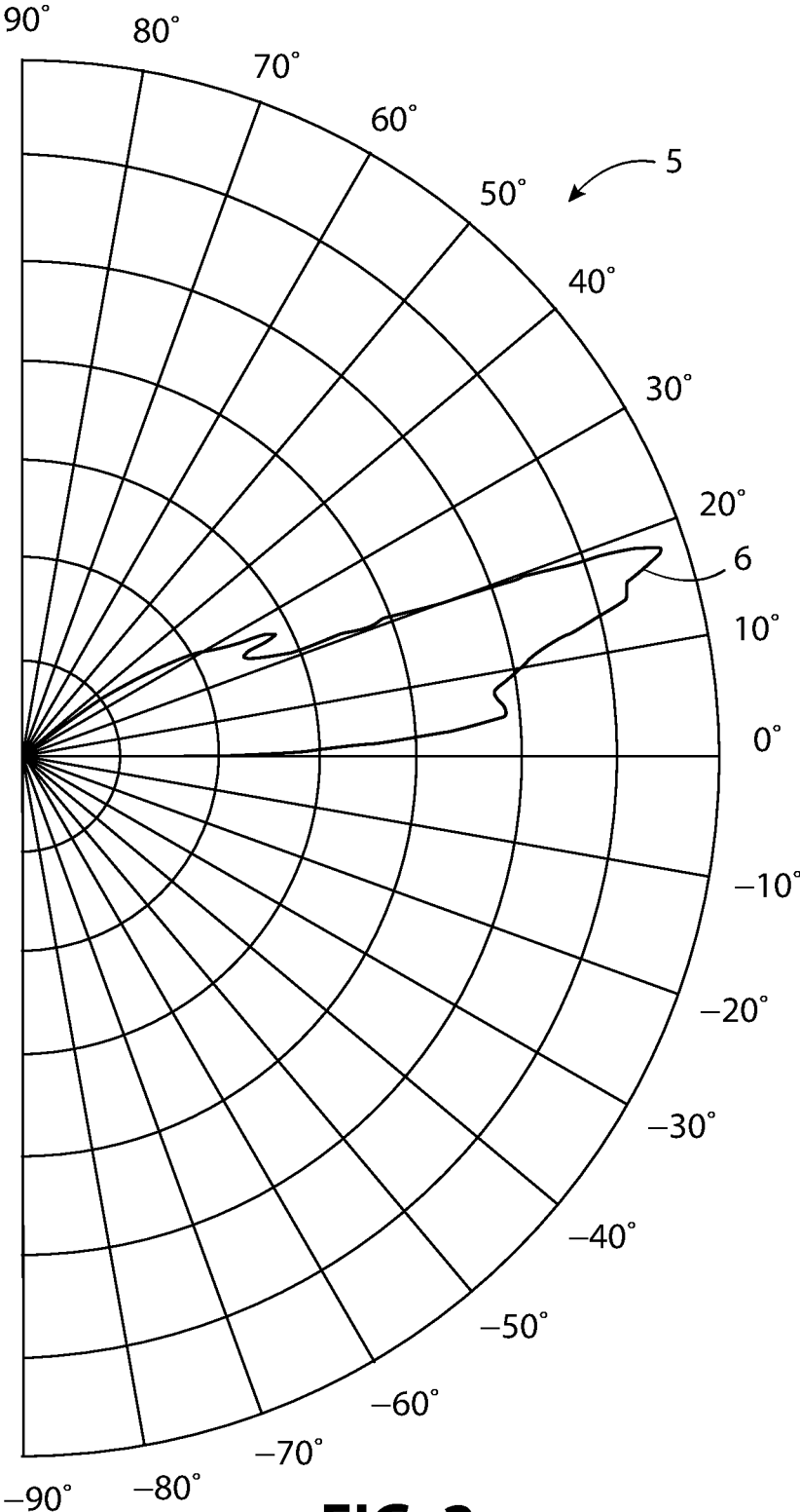
FIG. 2 PRIOR ART
