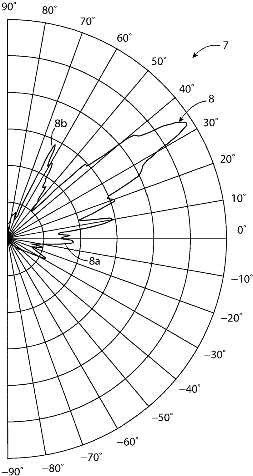
FIG. 3 PRIOR ART
