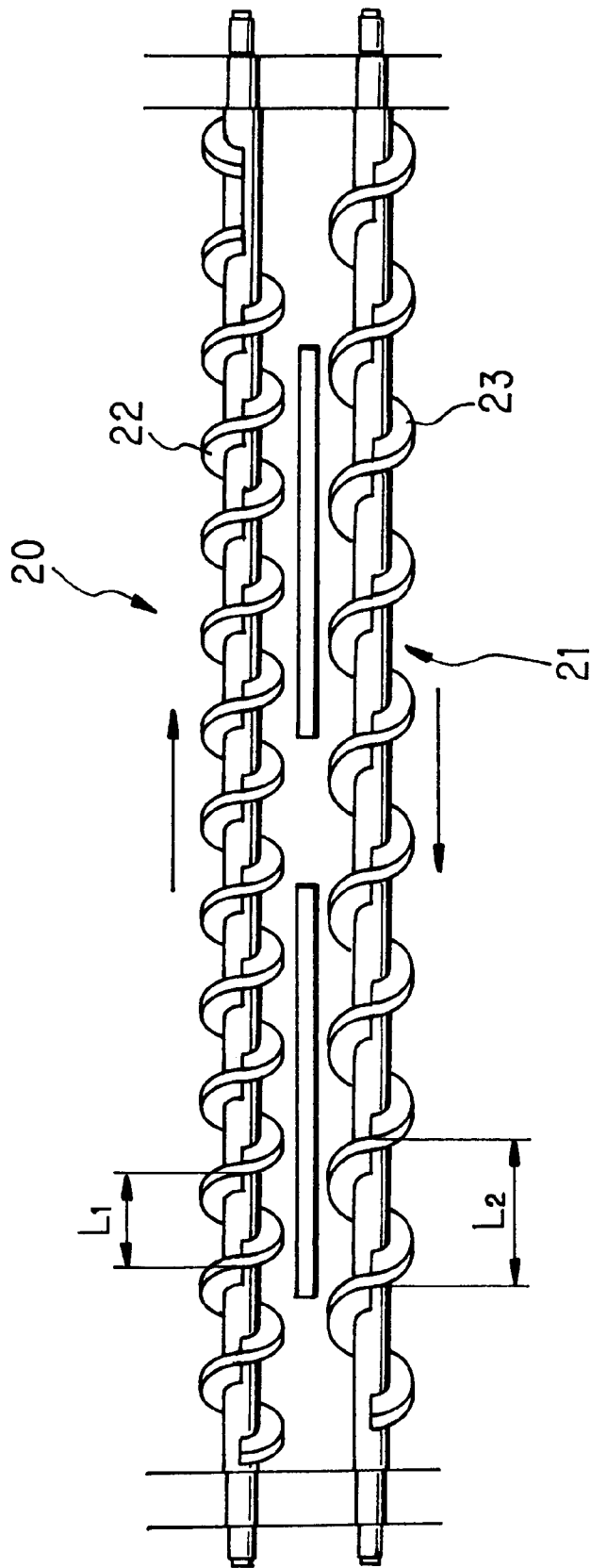
FIG. 3 PRIOR ART
