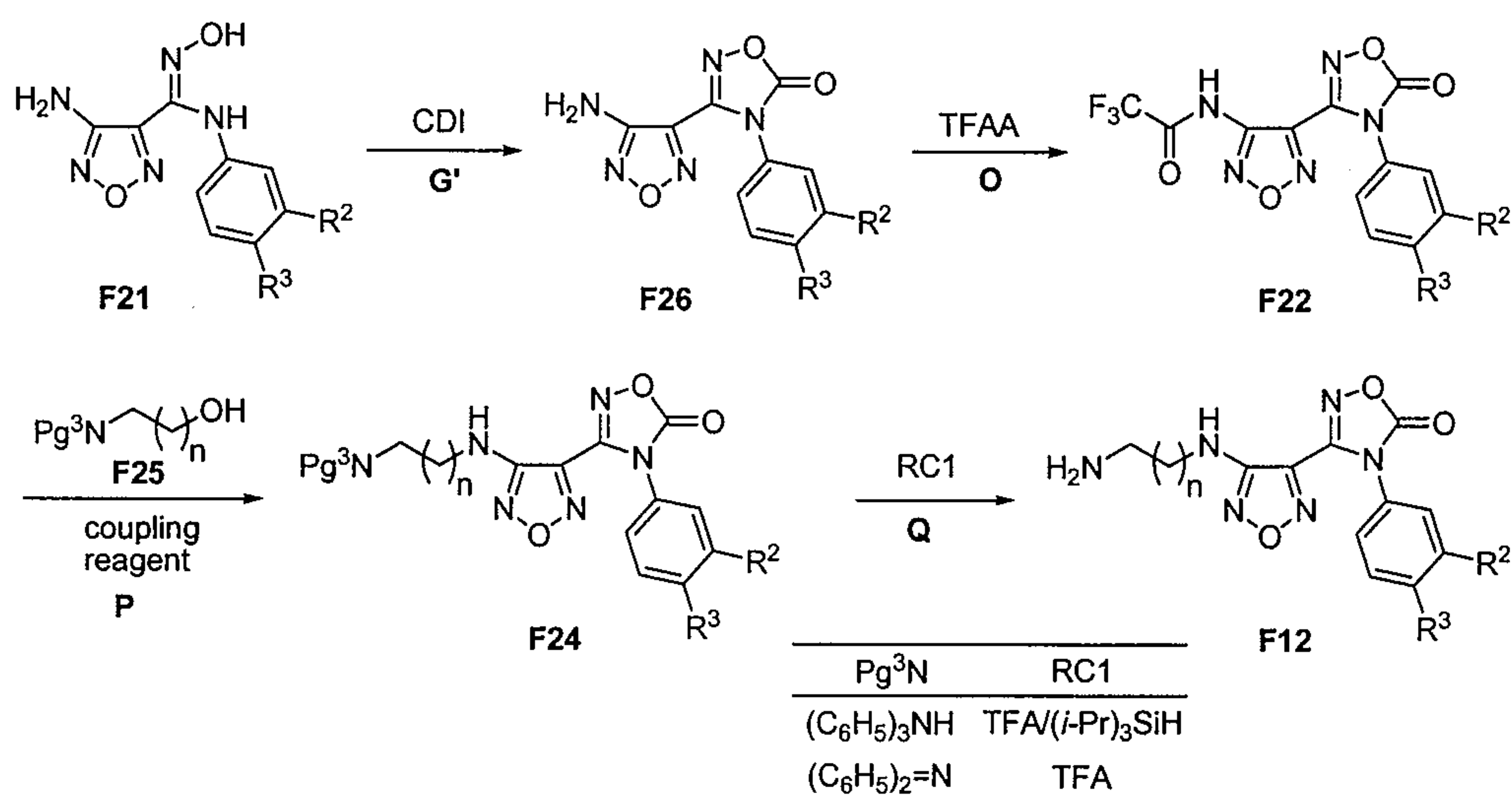
Scheme 4
