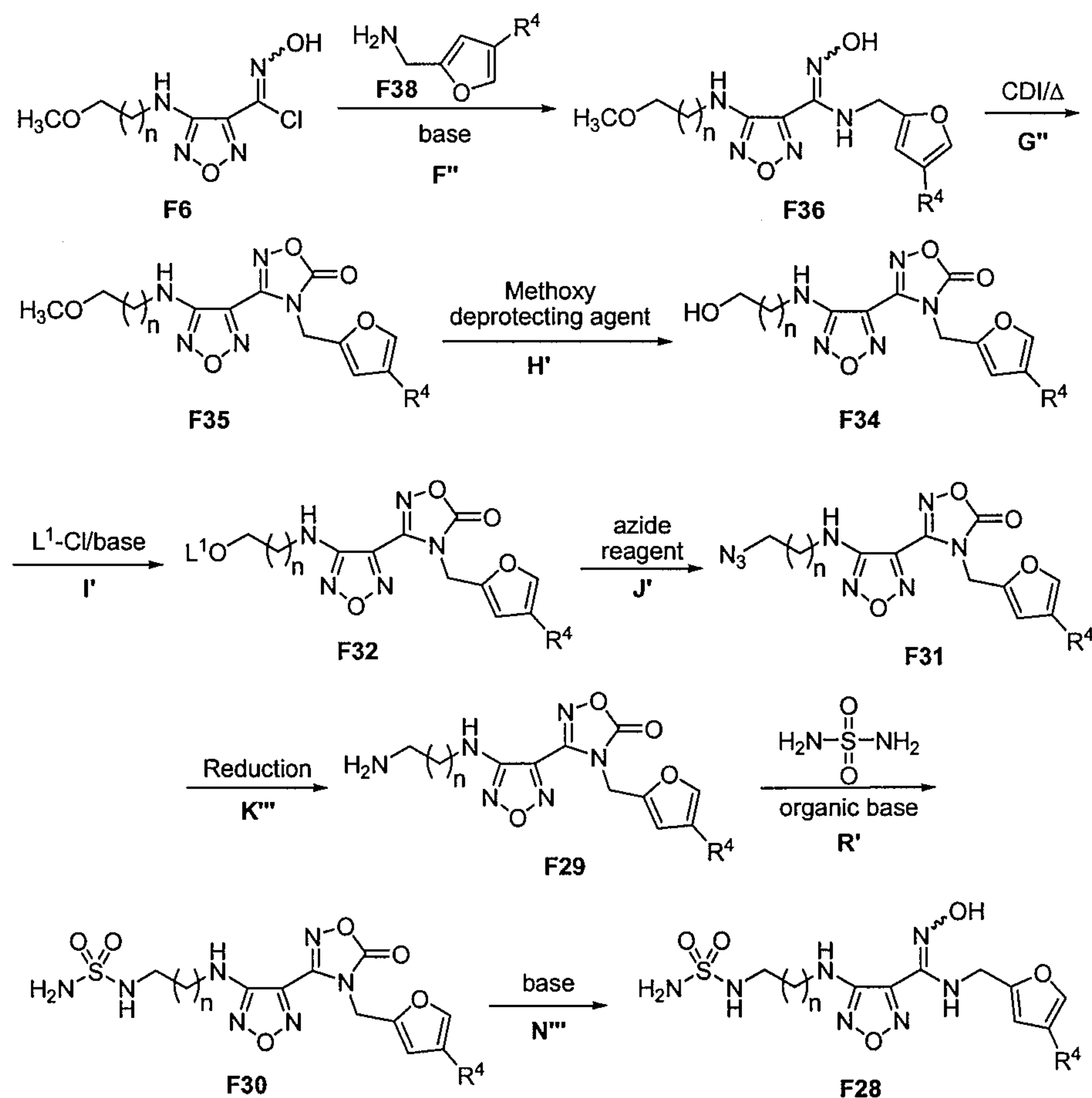
Scheme 9
