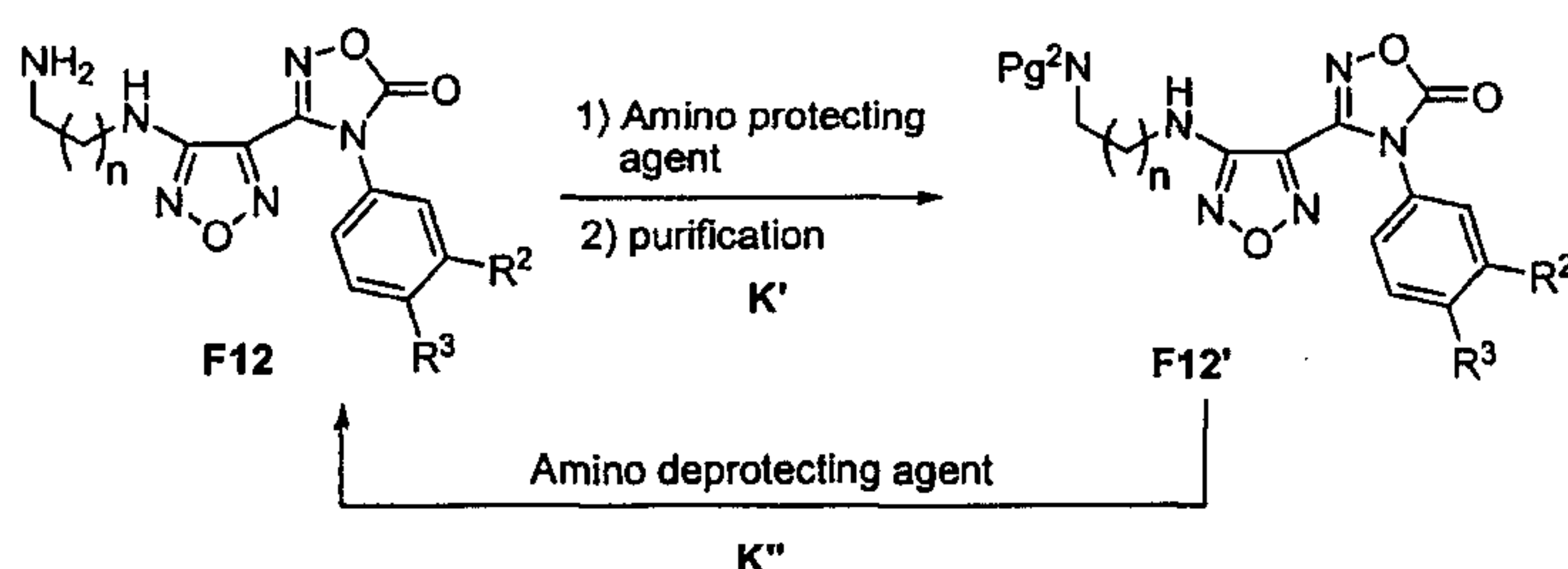
Scheme 2
