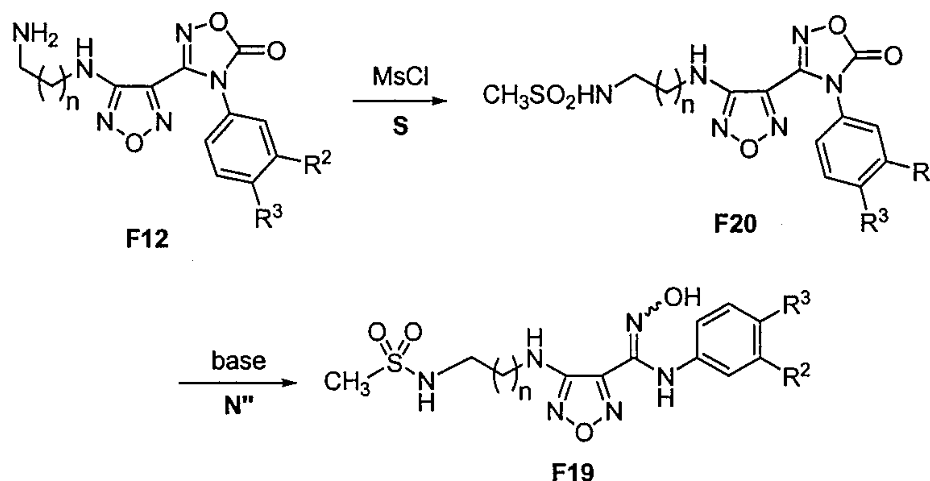
Scheme 7
