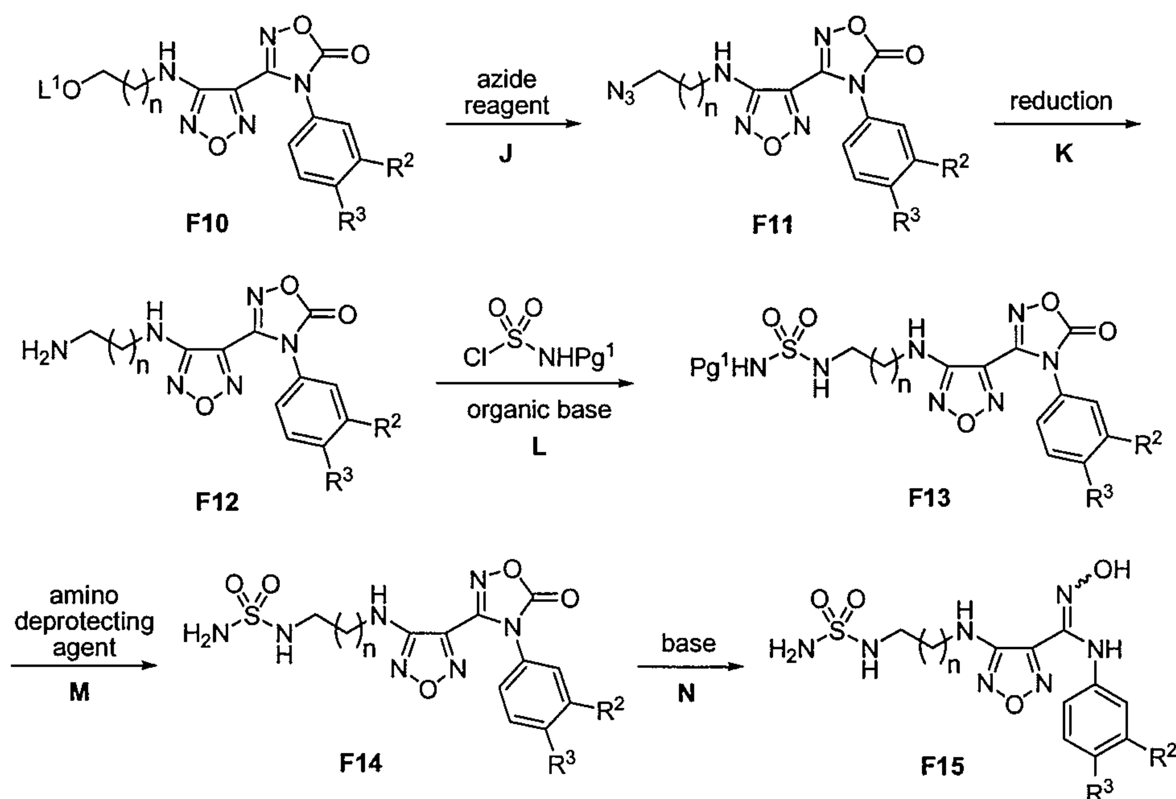
Scheme 1
