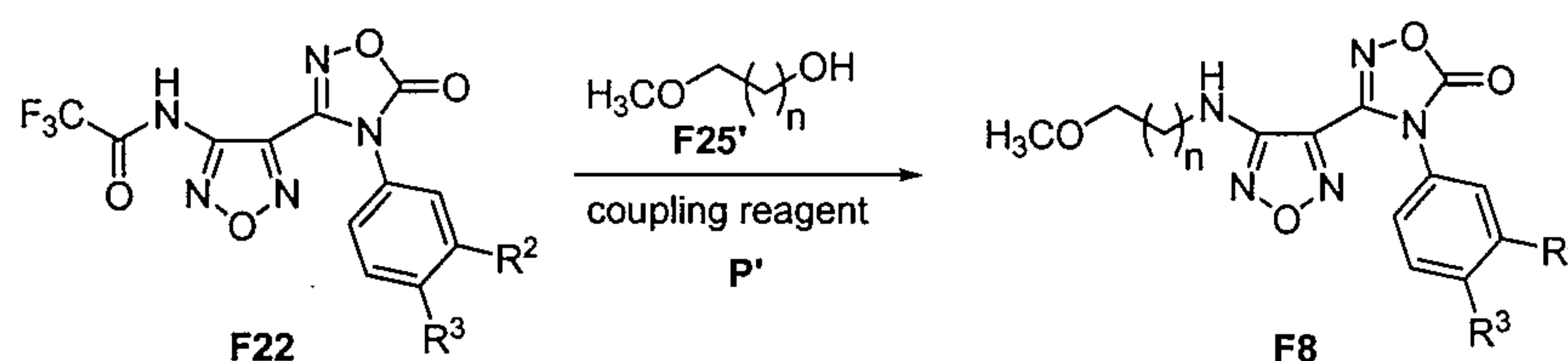
Scheme 5
