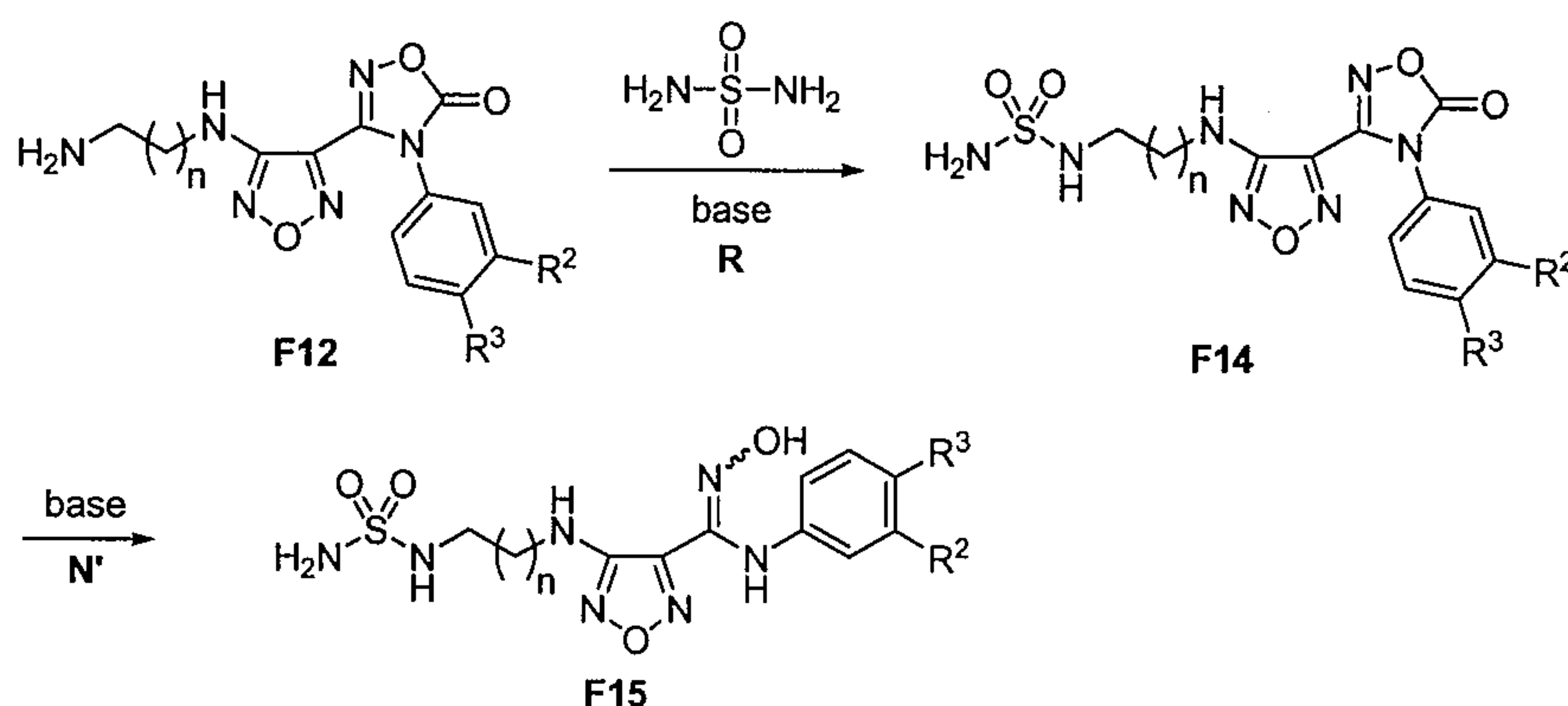
Scheme 6
