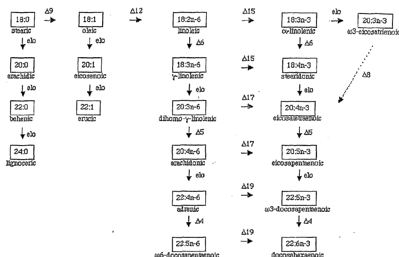
Figure 1 Fatty Acid Biosynthetic Pathway
