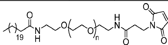
PEG5K+C22
