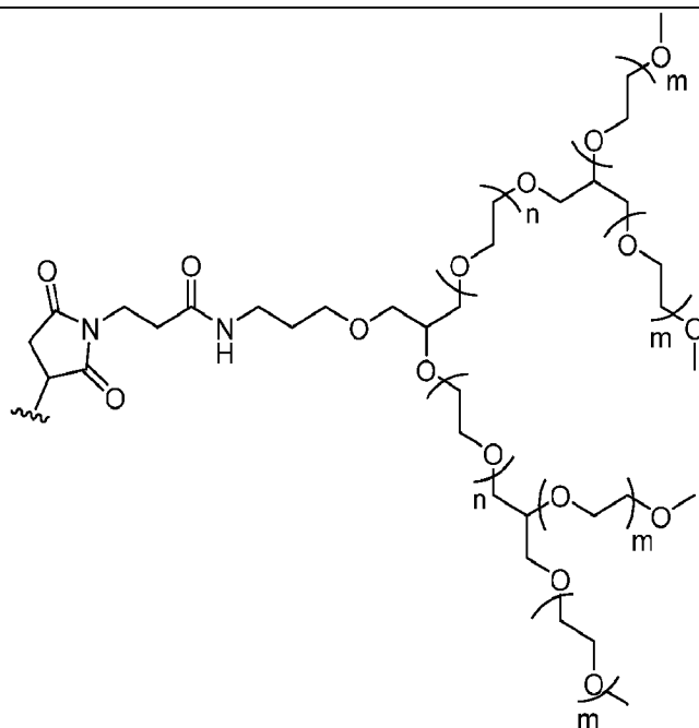
PEG40K (2x2-arm),
