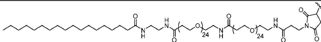
PEG48+C18
