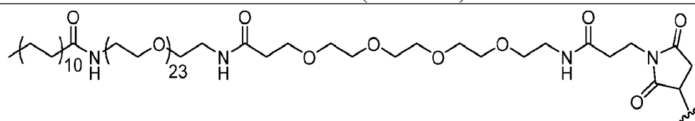
PEG23+C22
