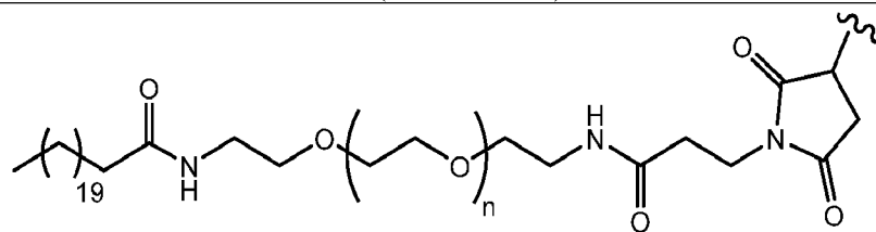
PEG5K+C22
