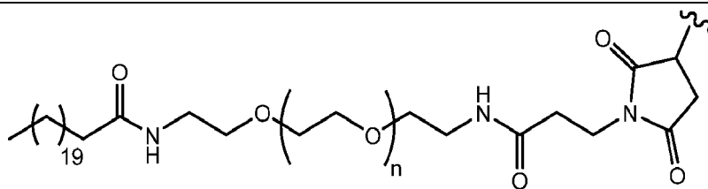
PEG5K+C22
