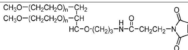
PEG40K (2-arm),
