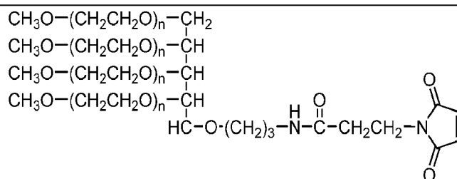
PEG40K (4-arm),
