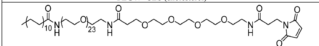
PEG23+C22
