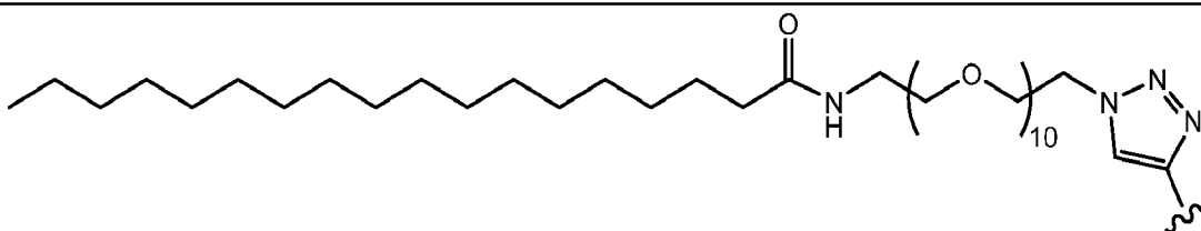
C18
