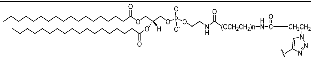
DSPE-PEG5K-N3
