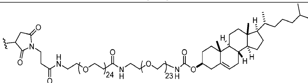
PEG47+CLS (cholesterol)
