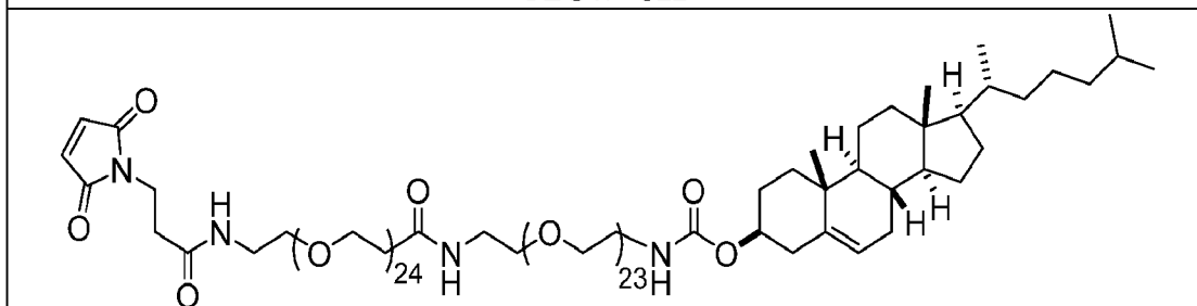
PEG47+CLS (cholesterol)
