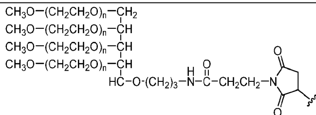
PEG40K (4-arm),
