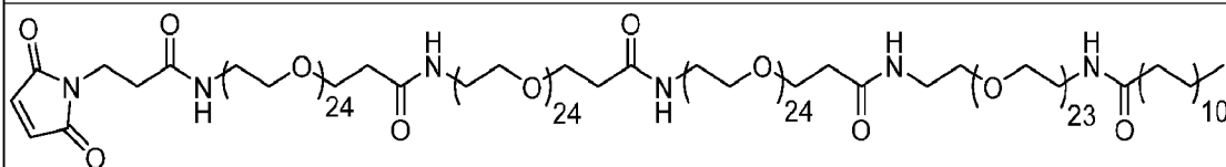
PEG95+C22
