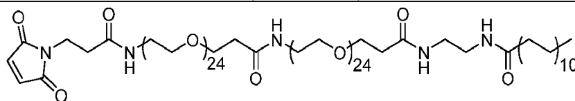
PEG48+C22
