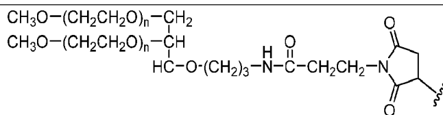
PEG40K (2-arm),
