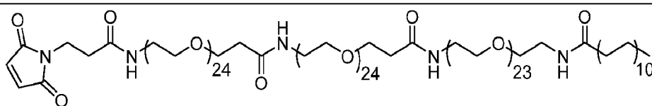
PEG71+C22
