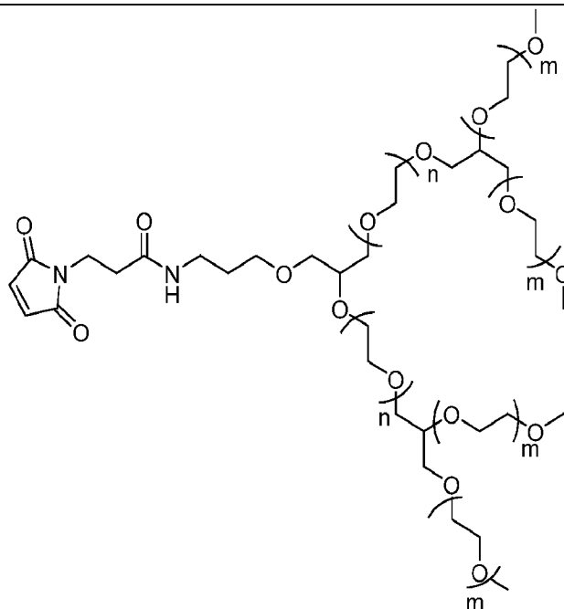
PEG40K (2x2-arm),
