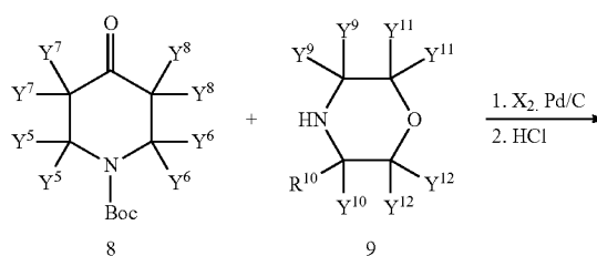
Scheme 2. Preparation of Intermediate 6.
