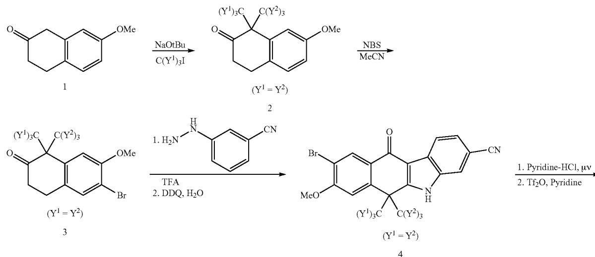
Scheme 1. Preparation of a Compound of Formula I.
