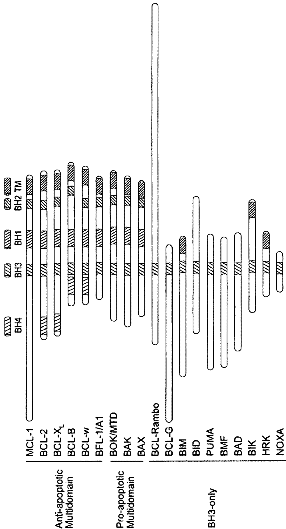
BCL-2 family members share conserved BCL-2 homology (BH) domains.
