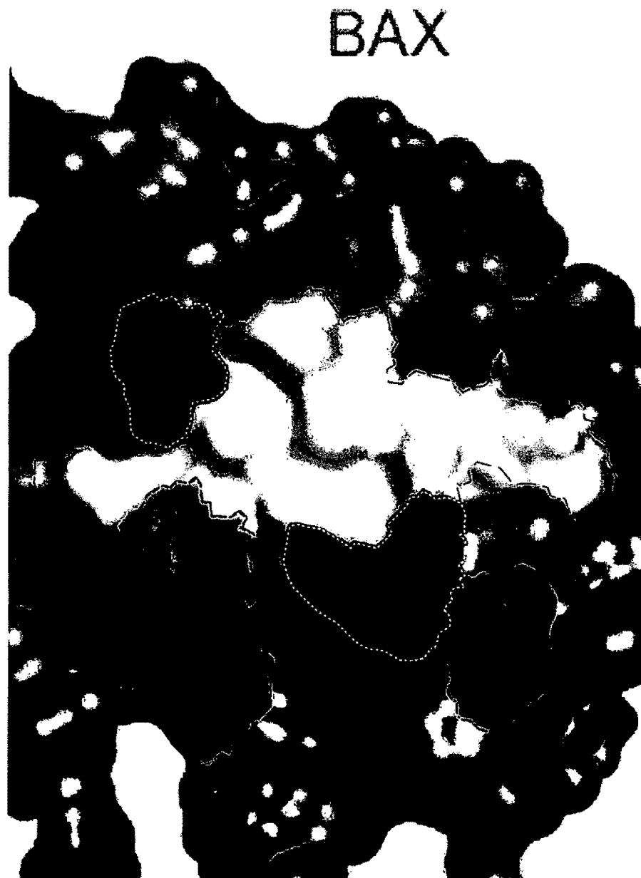
BH3 Interaction site on BAX
