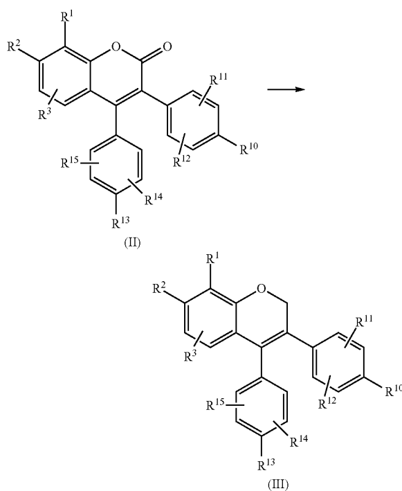
Scheme 3: Preparation of a functionalized chromene
