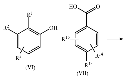
Scheme 1: Preparation of a benzophenone intermediate
