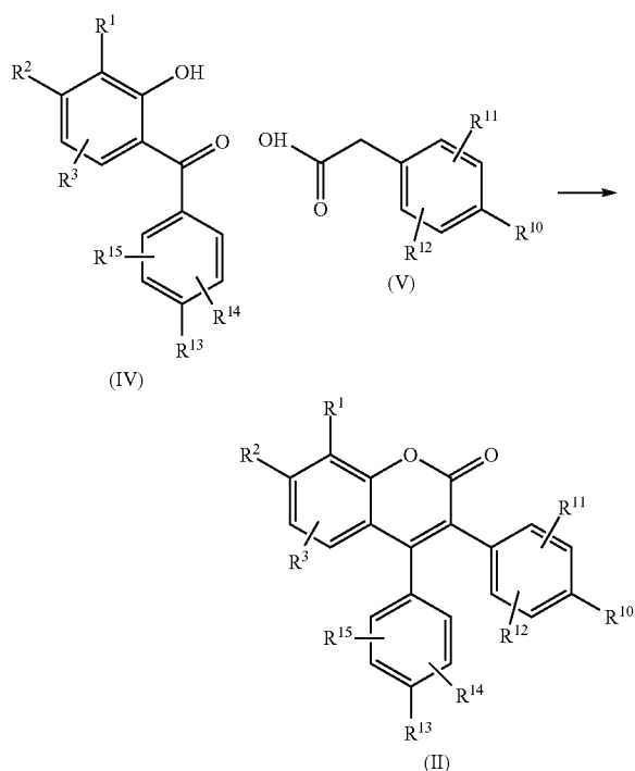
Scheme 2: Preparation of a functionalized benzopyranone
