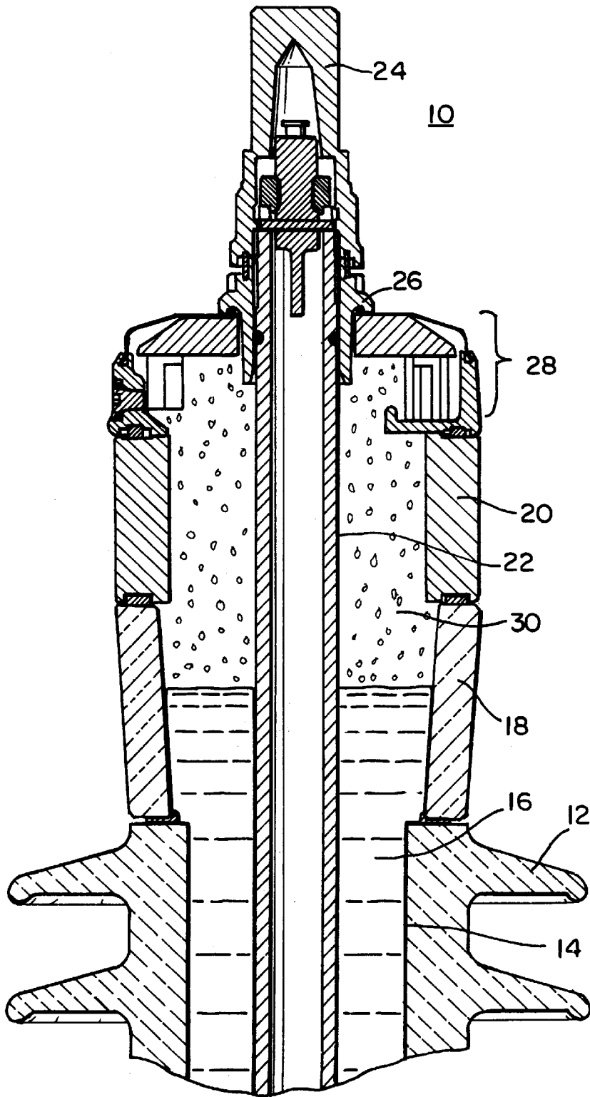
FIG. 1 PRIOR ART
