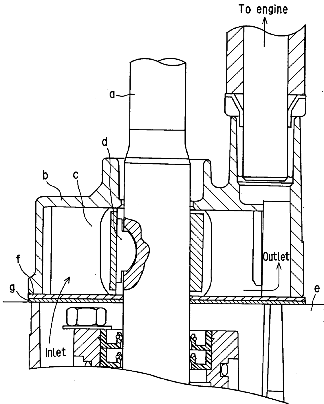
Conventional stainless cooling pump configuration
