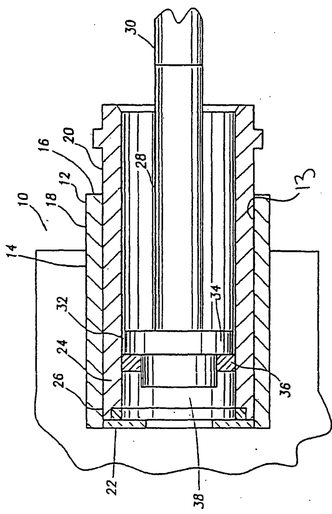
FIG. 1 (PRIOR ART)
