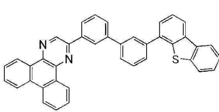
2mDBTBPDBq-II
