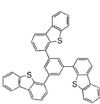
DBT3P-II
