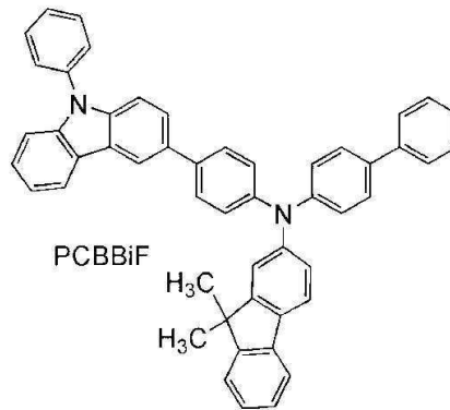
BPAFLP
