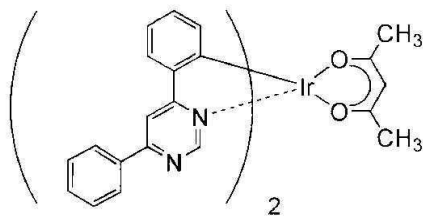
[Ir(dppm) 2 (acac)]
