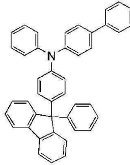
BPAFLP
