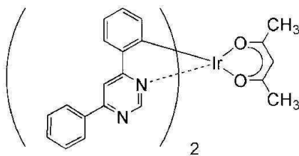
[Ir(dppm) 2 (acac)]
