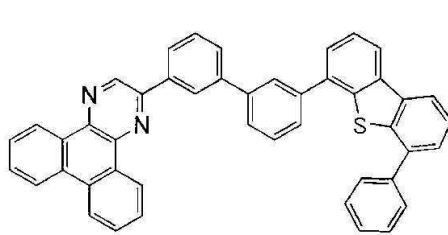
2mDBTBPDq-IV
