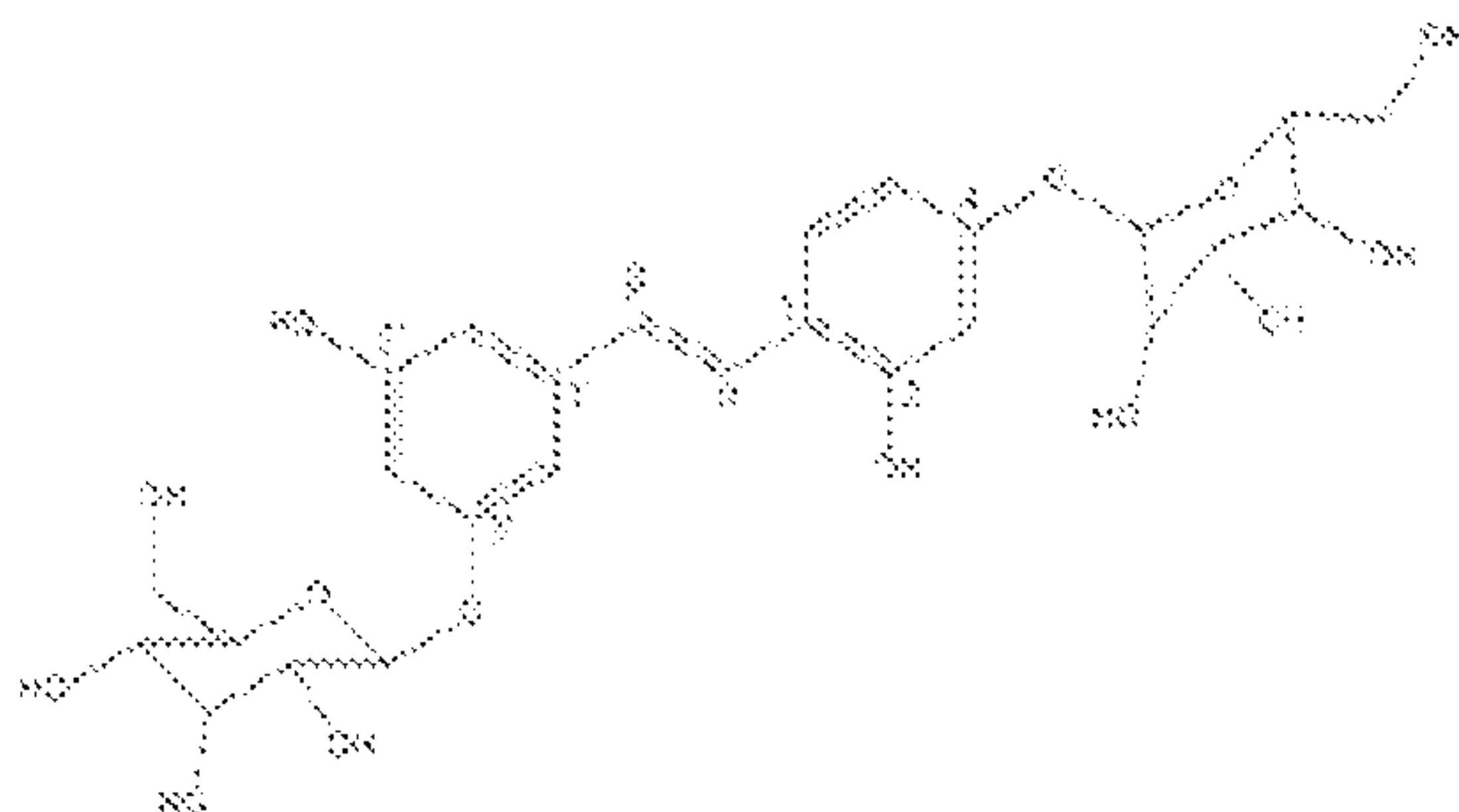
Mulberroside A
