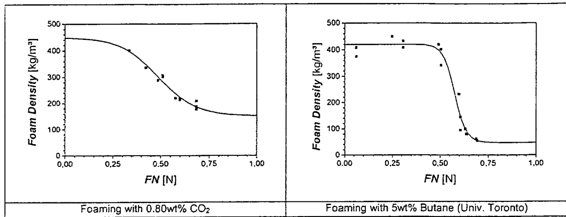
Figure 2: Correlation for minimum foam density and Foamability Number - with FN > 0.30 low density foam is achieved (< 400 kg/m 3 )
