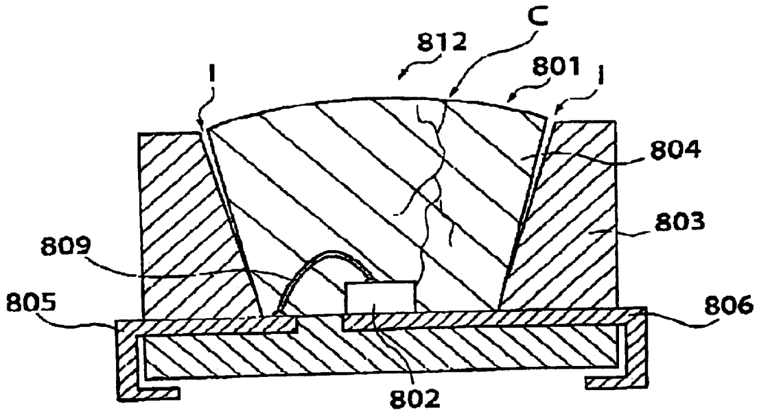
FIG. 38 Prior Art
