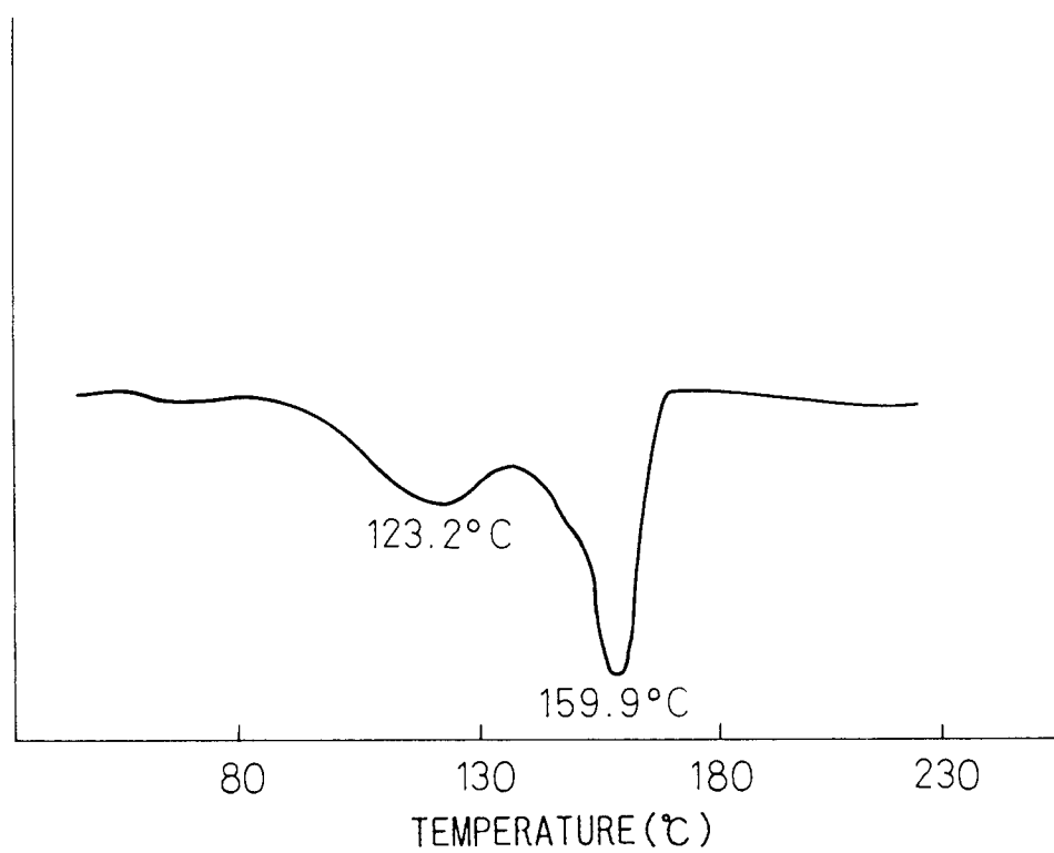
Fig.13 DSC CHART (EXAMPLE 7)
