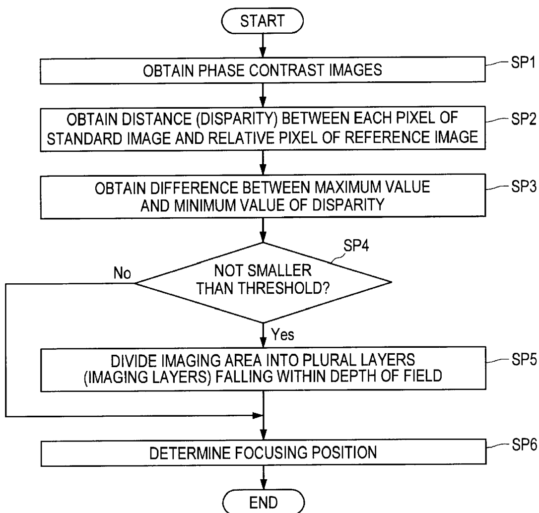
FOCUSING POSITION DETERMINATION PROCEDURE
