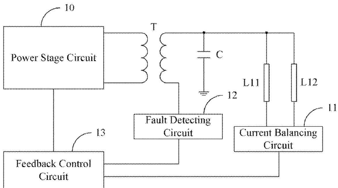
FIG. 6 (Related Art)
