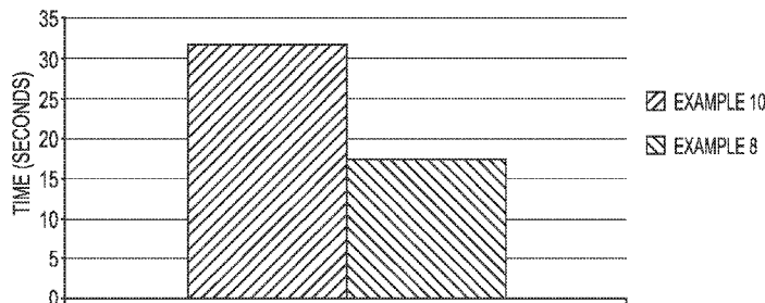
BURN - THROUGH TIME OF 0.77% AQUEOUS DISPERSIONS IN 460 mg/L CALCIUM CARBONATE HARDNESS WATER
