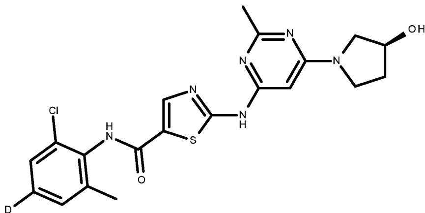
compound IV
