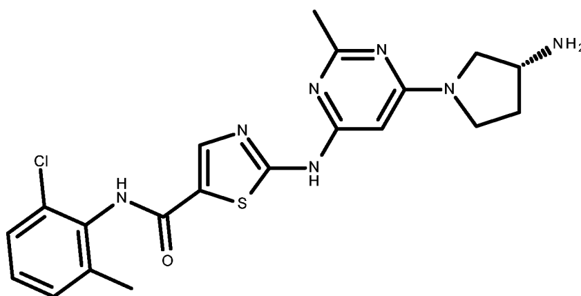
compound XIII
