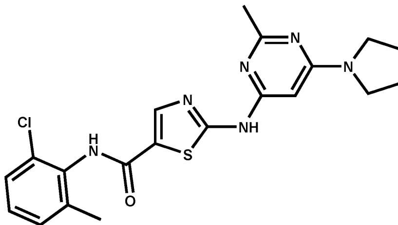
compound XIV
