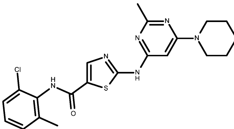
compound VIII
