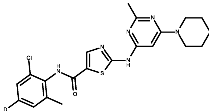
compound I
