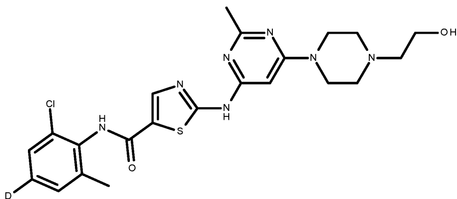
compound III
