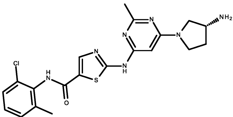
compound XIII
