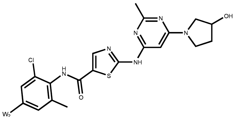
formula IV
