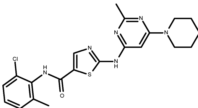
Compound VIII
