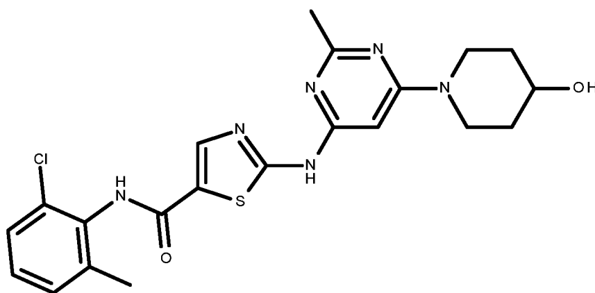
compound IX
