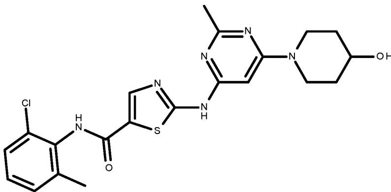
compound IX
