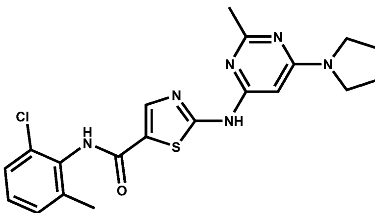
compound XIV
