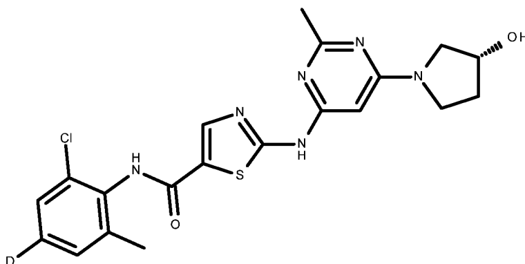
compound V
