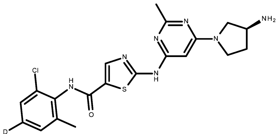
compound VI
