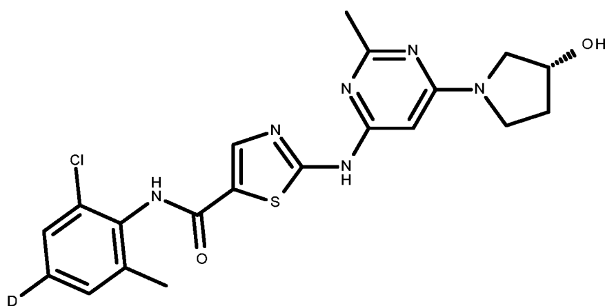
compound V
