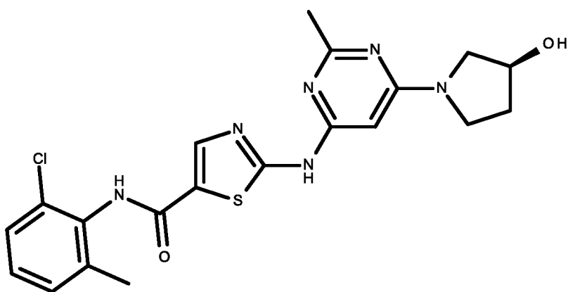
compound X
