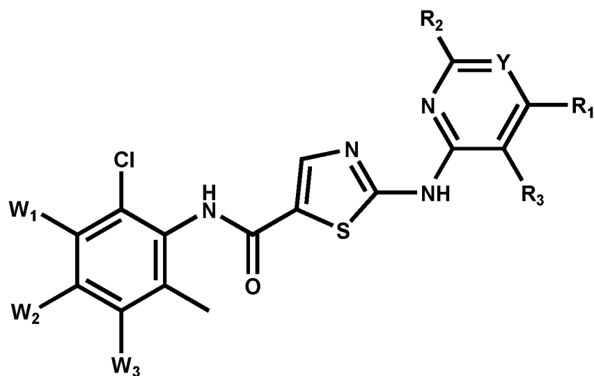
formula I
