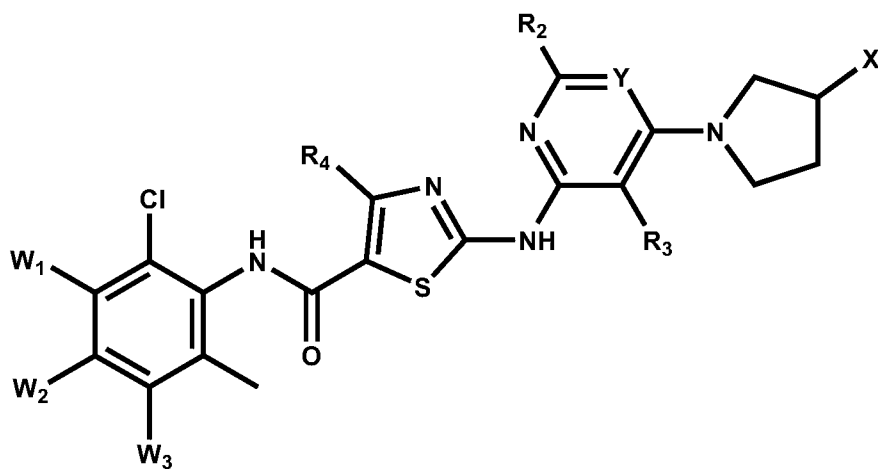
formula II
