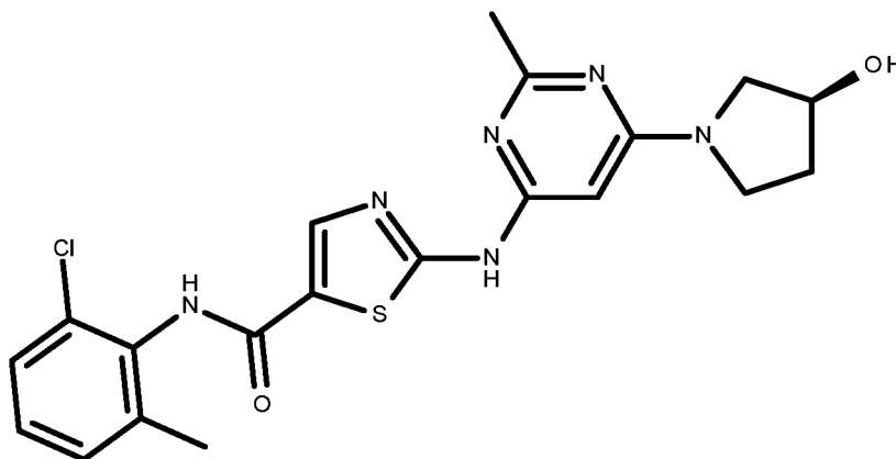
compound X
