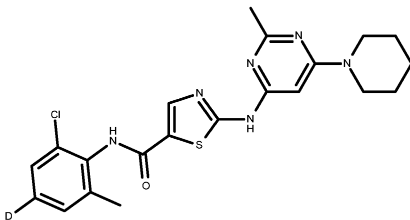
compound I
