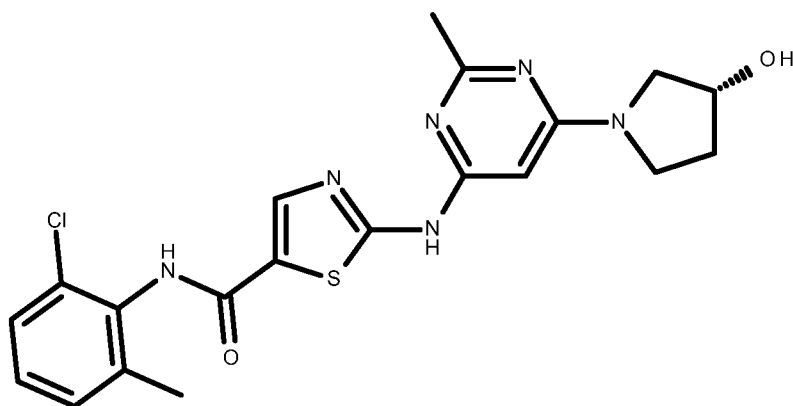
compound XI
