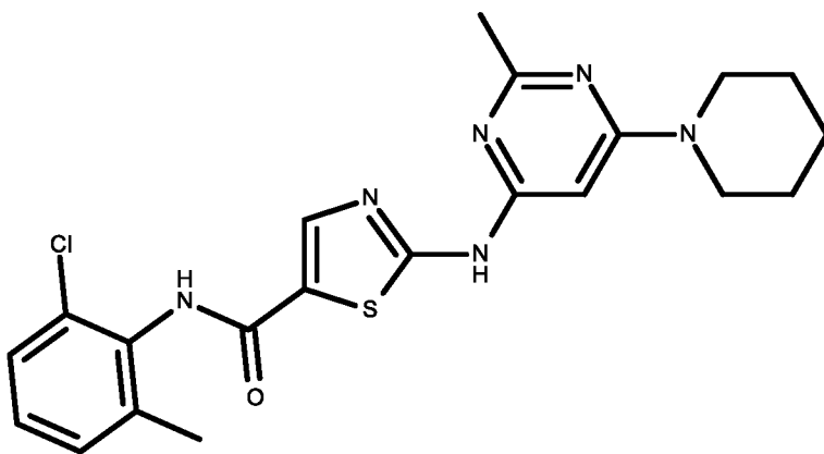
compound VIII
