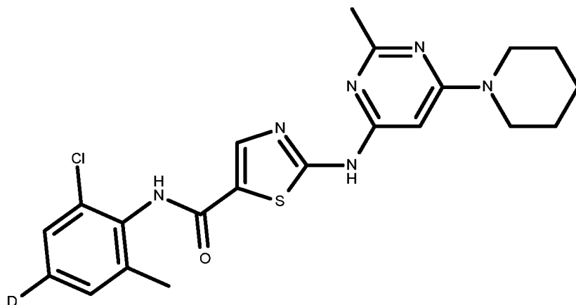
compound I
