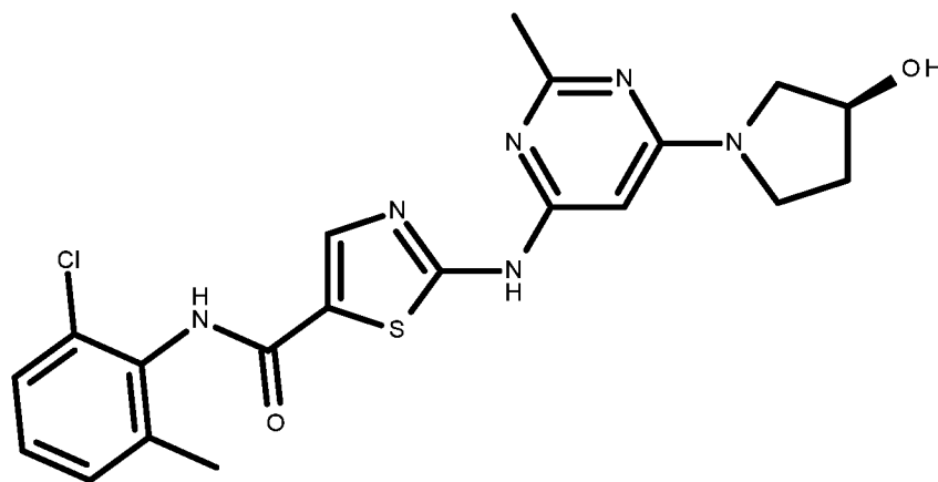
compound X
