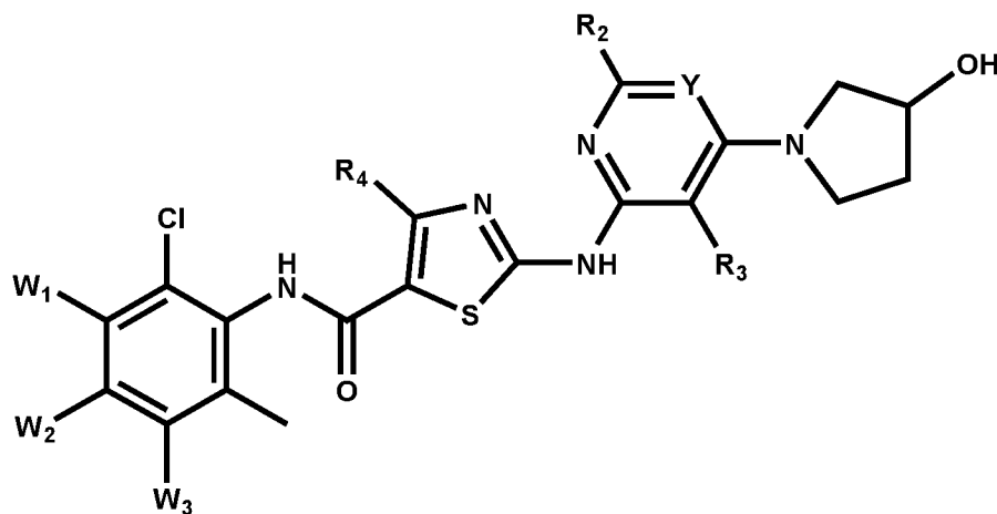
formula III
