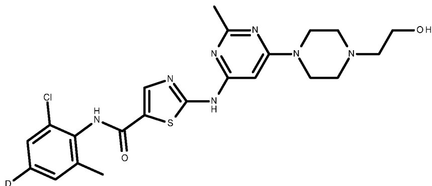
compound III
