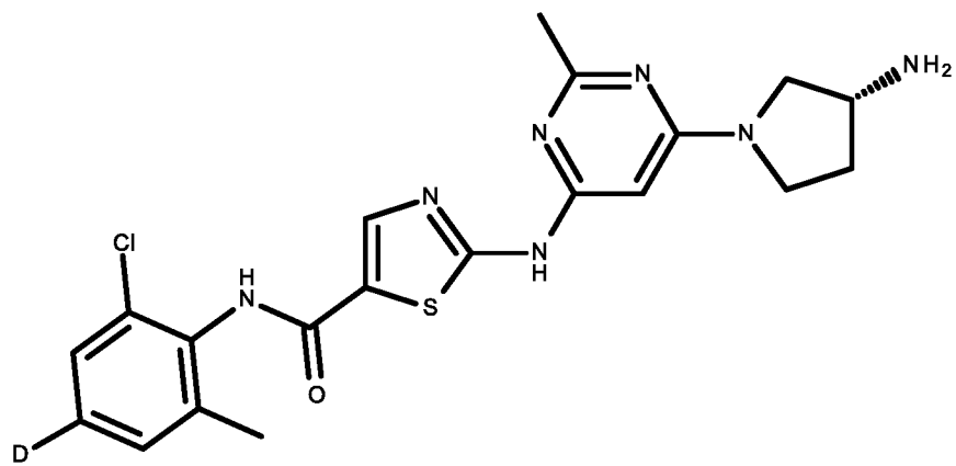
compound VII
