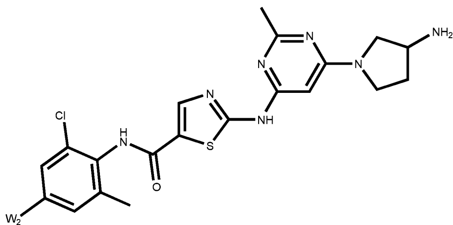
formula V
