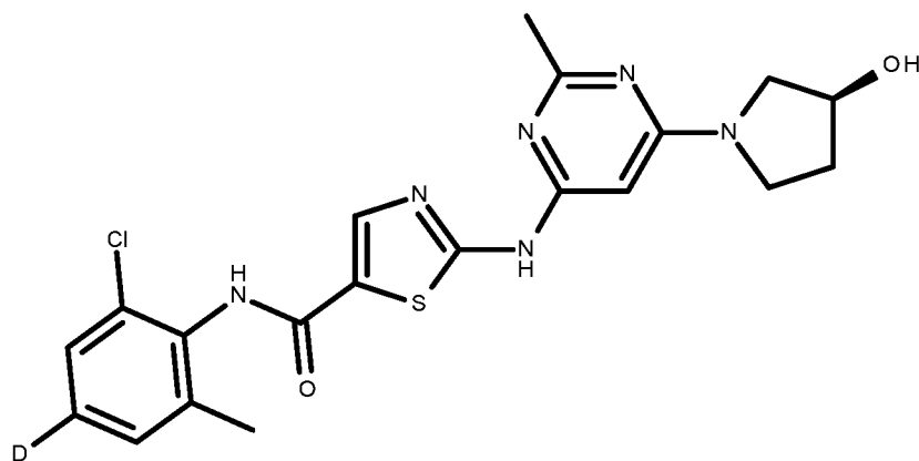
compound IV
