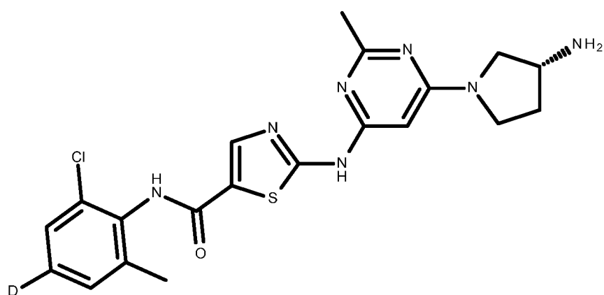
compound VII
