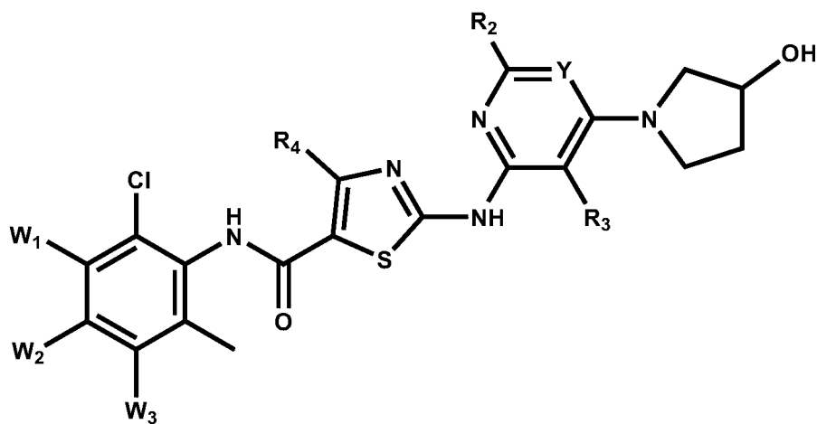
formula III
