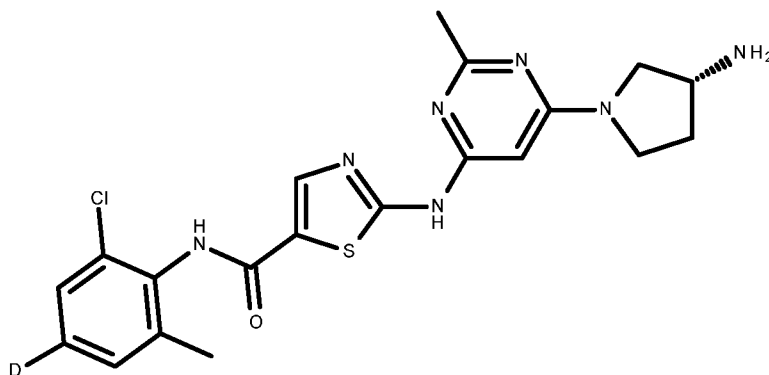
compound VII
