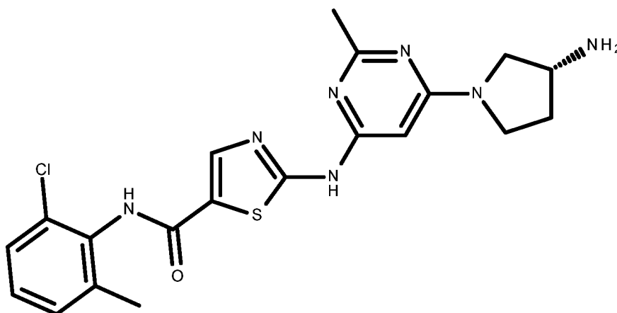
compound XIII
