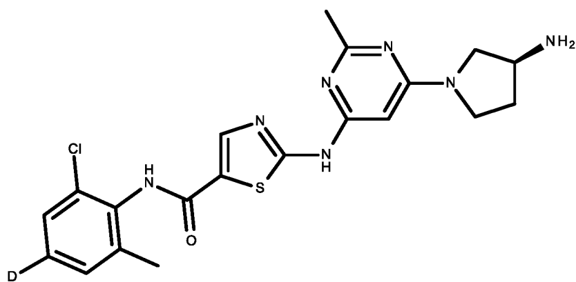
compound VI
