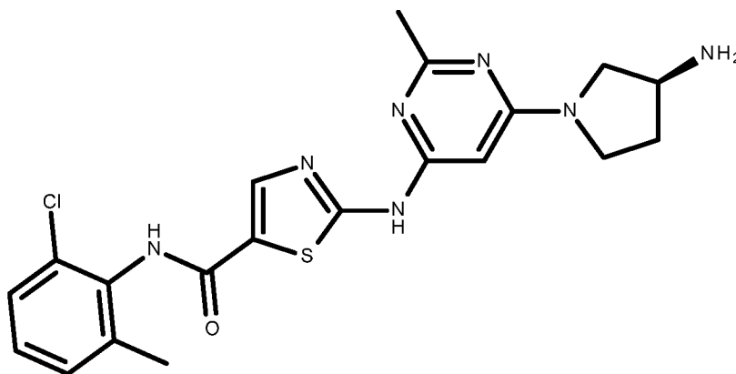
compound XII
