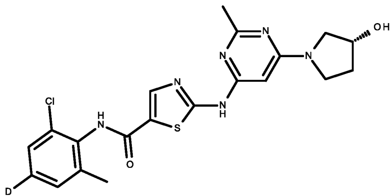
compound V
