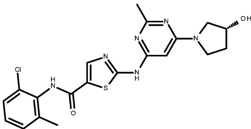
compound XI
