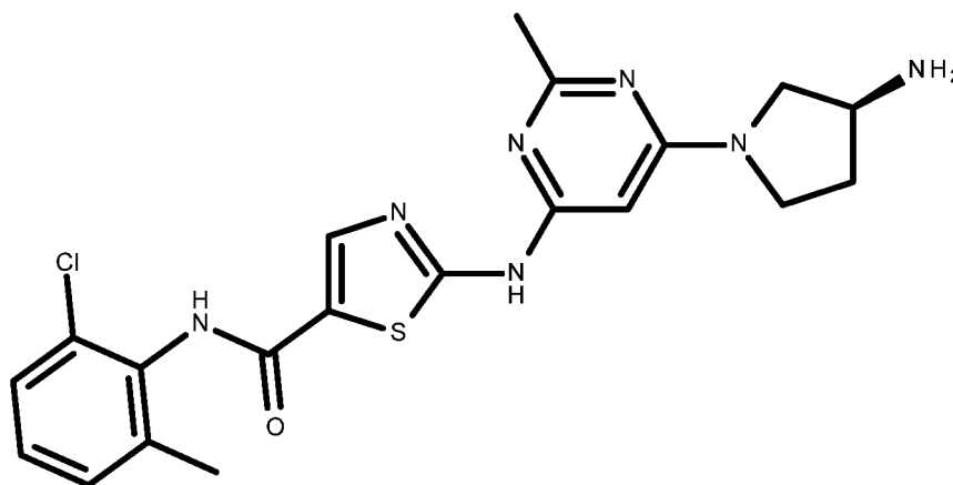
compound XII
