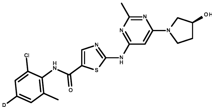
compound IV
