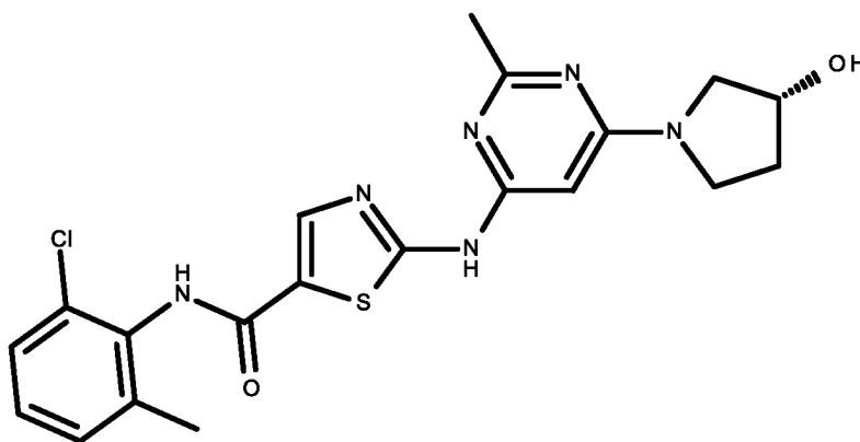
compound XI
