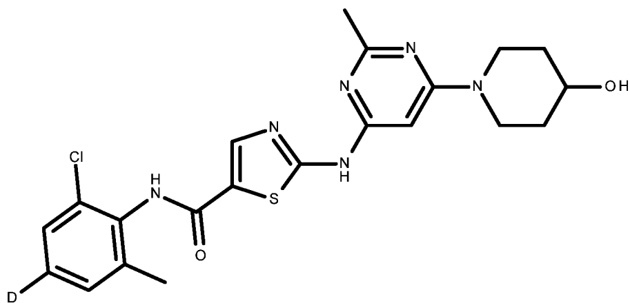
compound II
