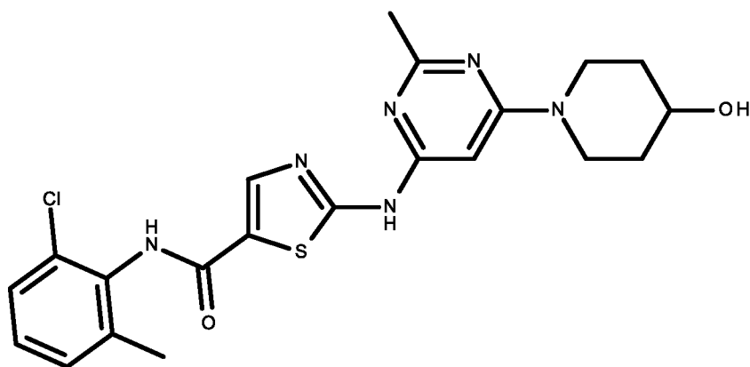
compound IX
