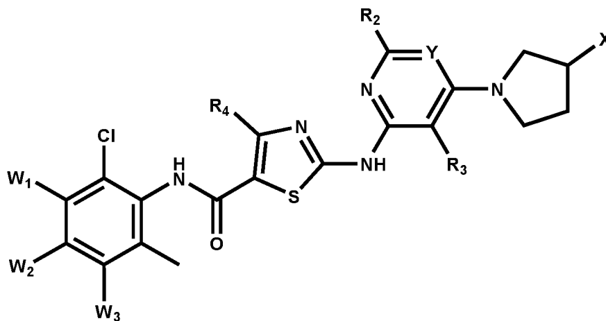
formula II
