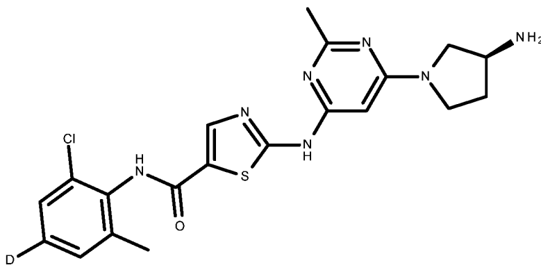
compound VI
