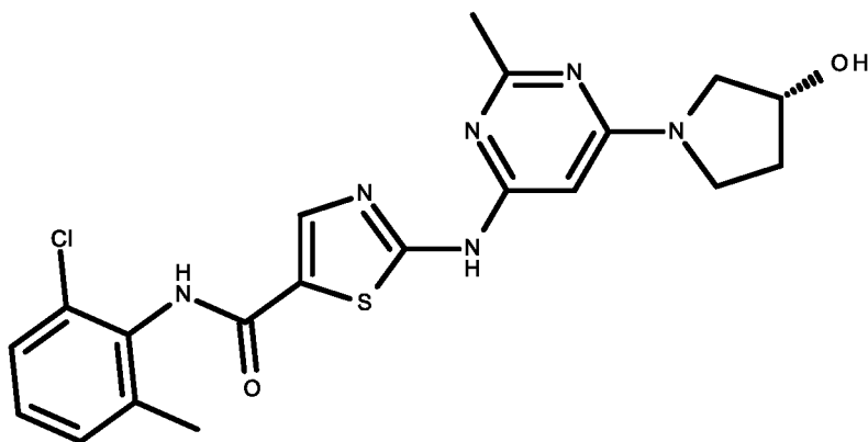
compound XI
