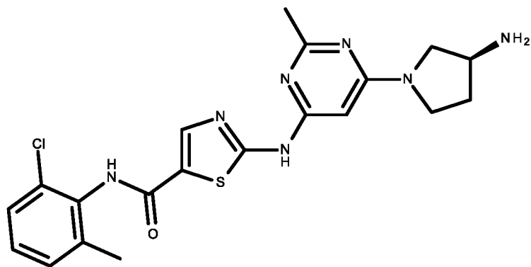
compound XII
