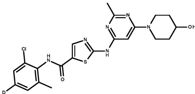
compound II
