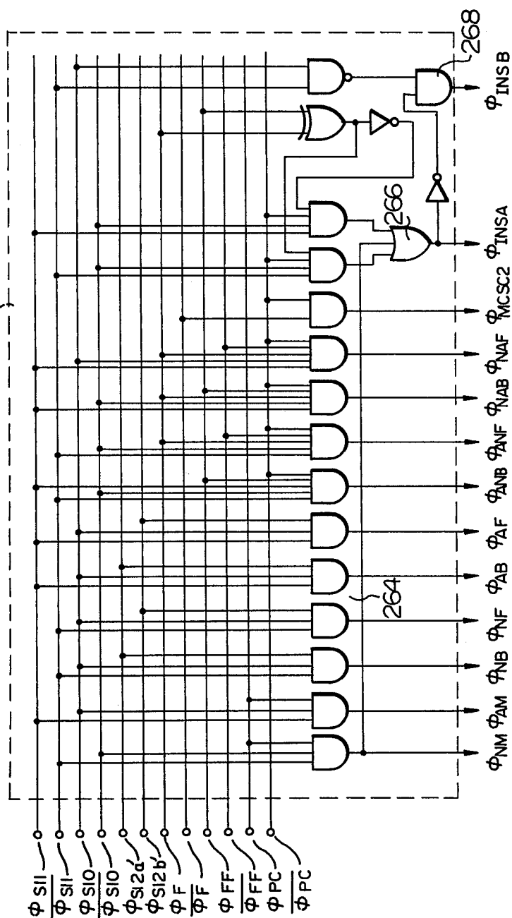
Fig. 18 OPERATION SELECTION CIRCUIT 252
