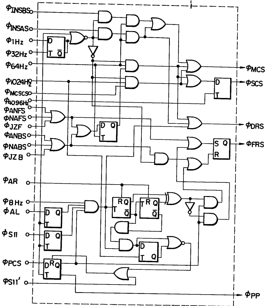
SECONDS CHANGEOVER CONTROL CIRCUIT 334
