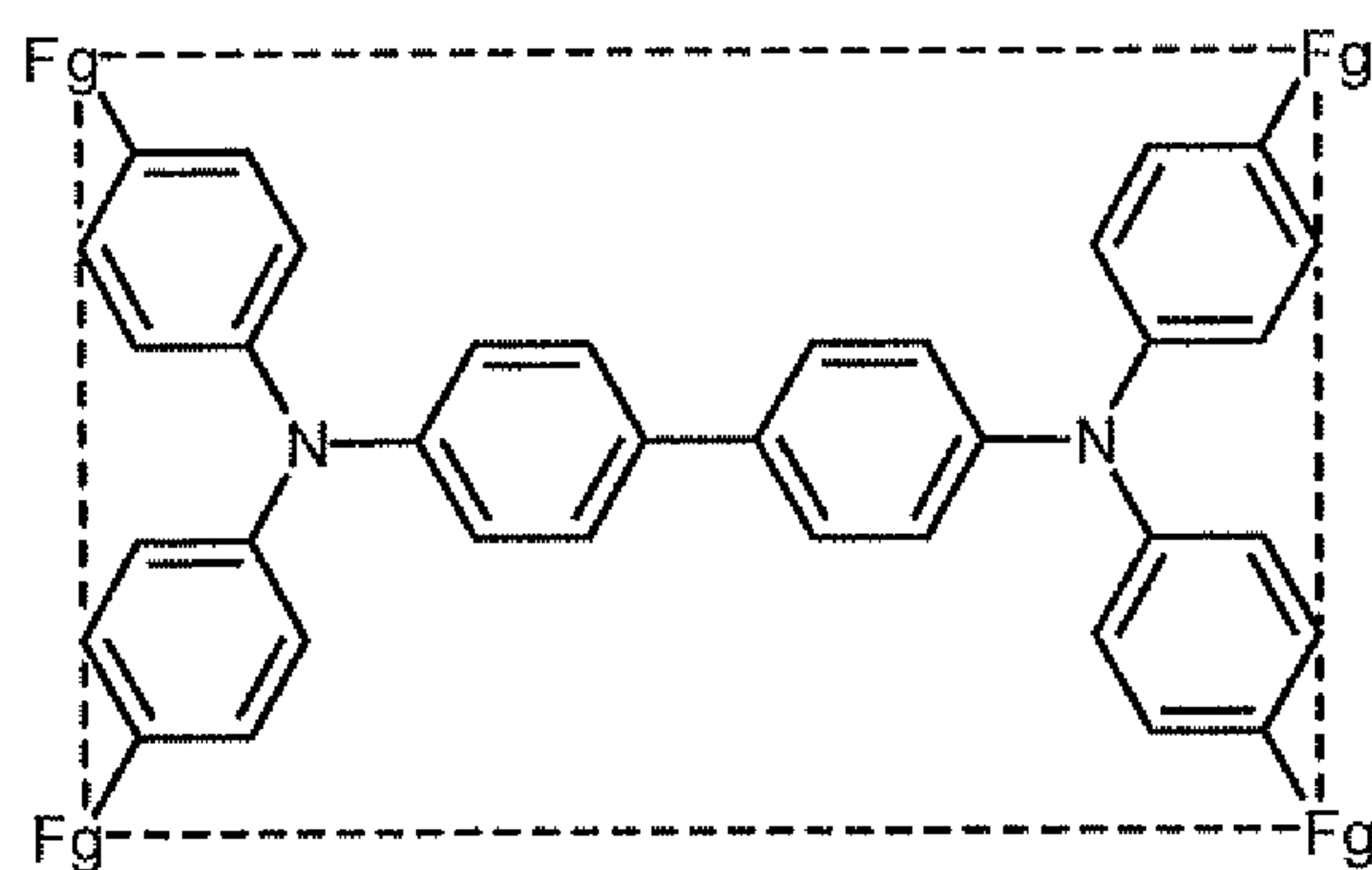
distorted square/tetrahedra building block ,
