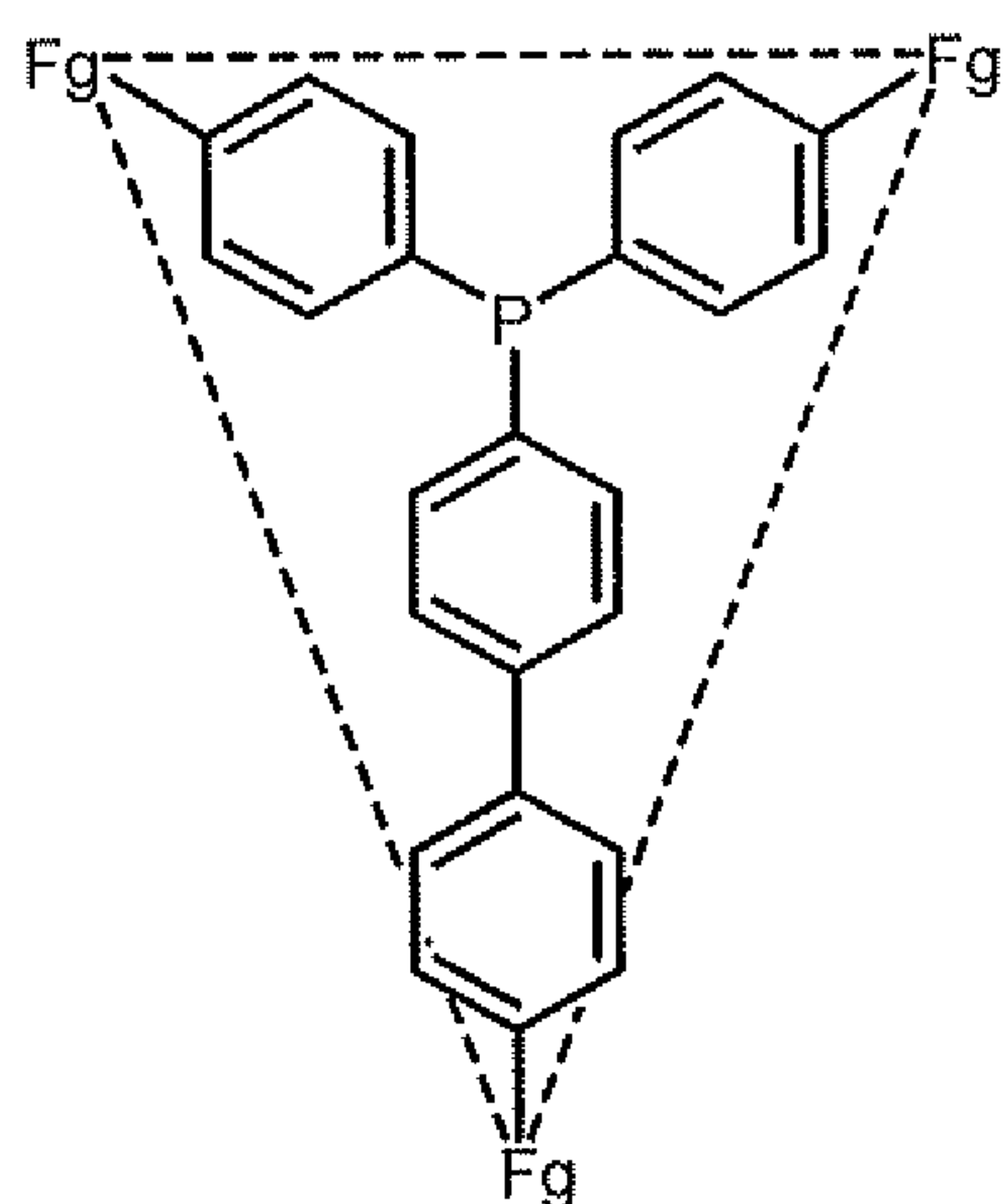
distorted triangular building block , distorted triangular building block
