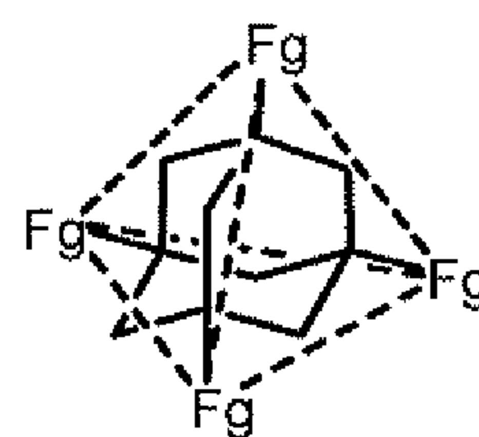
ideal tetrahedral building block ,
